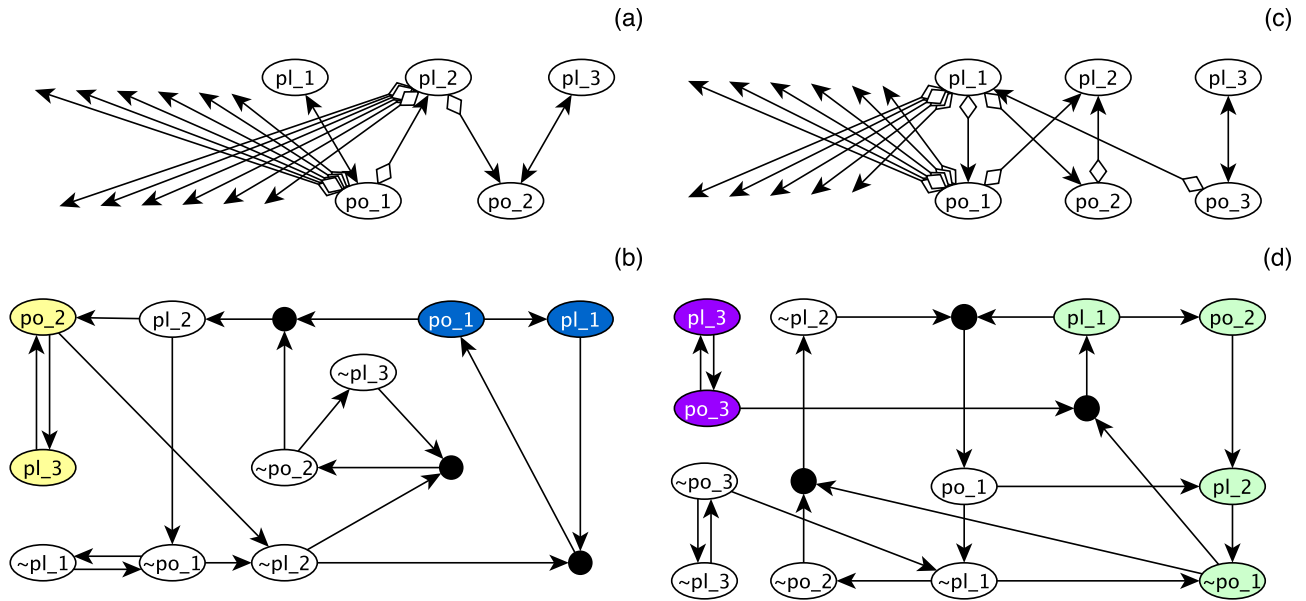
FIG. 14. The simplest subnetworks that can yield supported active or mixed-state CSMs. Panel (a) shows a subnetwork that has 9 plants and 8 pollinators. Nodes pl_2 and po_1 each have 1 positive and 7 negative incoming edges. For each of these nodes the starting point of 6 incoming negative edges can be arbitrary nodes outside of the nodes with labels. Only one of the negative incoming edges is kept during network simplification. A single case among 49 possible choices, namely, keeping the negative edges from po_2 to pl_2 and from pl_2 to po_1 results in a network consisting of pl_1 , pl_2 , pl_3 , po_1 , and po_2 that is capable of forming a supported active CSM. Panel (b) shows the corresponding expanded network. The yellow SM consisting of po_2 and pl_3 is the support of the blue active CSM. Panel (c) shows a subnetwork that has the same number of plants and pollinators. Keeping the negative edges from po_1 to pl_1 and from pl_2 to po_1 results in a simplified network that has a mixed-state CSM, highlighted with green in the expanded network of panel (d). The purple SM consisting of pl_3 and po_3 is the support of this mixed state CSM. This case has the same probability of 1 in 49 choices.
