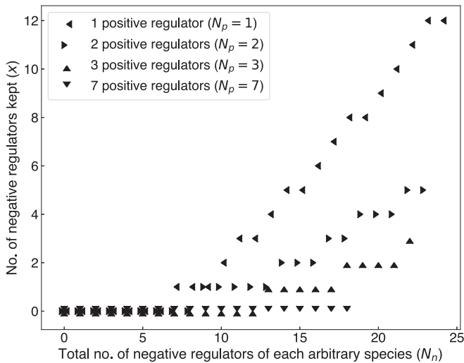
FIG. 11. The number of negative regulators of each arbitrary species that are kept after the simplification according to Eq. (B1). The figure shows examples of the number of negative regulators kept in the simplified model versus the total number of negative regulators in the threshold model, for four values of the number of positive regulators. According to the in-degree distributions in these networks, the maximum number of regulators a species can have is 25. As the number of positive regulators increases, the number of negative regulators they can overcome increases as well. Seven positive regulators can overcome 18 negative regulators, thus in this case there is no need to ensure the inactive state of any of the negative regulators.
