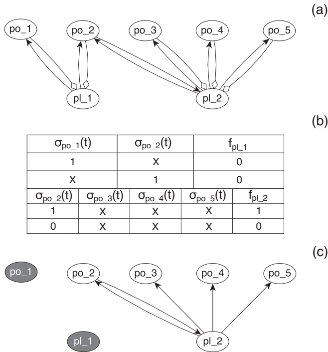
FIG. 2. A small plant-pollinator network depicting the mechanisms of edge loss when converting the threshold functions of the Campbell et al. model to disjunctive prime form. Panel (a) shows the bipartite network; plants are denoted with “pl” and pollinators are denoted with “po.” Edges with a regular arrowhead show positive influence, while edges with diamond arrowheads show negative influence on the target species. Panel (b) shows the truth tables for pl_1 and pl_2. The “X” in table entries means that the state of that particular species can be either 0 or 1. In this model, pl_1 becomes extinct because neither po_1 nor po_2 are able to pollinate it; this leads to the extinction of po_1. The future state of pl_2 depends only on the current state of po_2, because the weight of this positive influence is larger than the cumulative weight of the negative influences from po_3, po_4, and po_5. These observations allow us to simplify the network, as shown in panel (c), reducing computational complexity. The species that were not able to persist are highlighted with gray.
