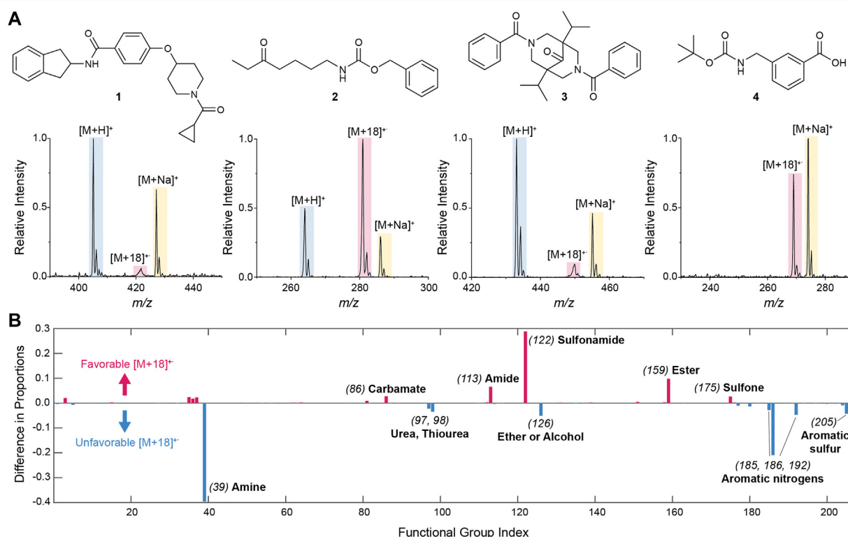
FIGURE 1 | (A) Representative examples of mass spectra from the 20,798-compound library showing cases of high and low [M+18]^+ intensity. Note the peak broadening in the low intensity cases. The structures of the molecules corresponding to the example spectra are also shown. (B) Effect of functional groups present in the molecule on the generation of [M+18]^+ as estimated from the difference in the proportion of compounds with a functional group within the set of [M+18]^+ hits and the same proportion in the complete library ( Supplementary Equation S3 ). A difference of zero indicates no effect of the functional group. Significant positive differences indicate that the formation of the [M+18]^+ species is favored by the presence of the functional group, whereas significant negative differences indicate a disfavoring effect. For the sake of simplicity, functional groups are indicated by indices specified in Supplementary Table S1 .
