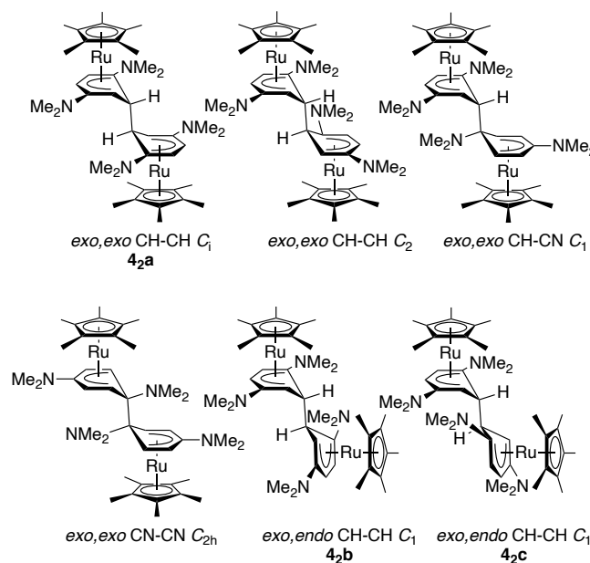
Scheme 5. Some isomers of [RuCp*(1,4-(Me 2 N)C 6 H 4 )] 2 , 4a , including all four possible exo,exo arene-arene isomers, one which ( 4a ) is isolated, and two of the possible exo,endo isomers ( 4b-c ), which are also isolated. All six of these are considered computationally (see Table 3). The highest symmetry point group that can be adopted by each isomer is indicated.
