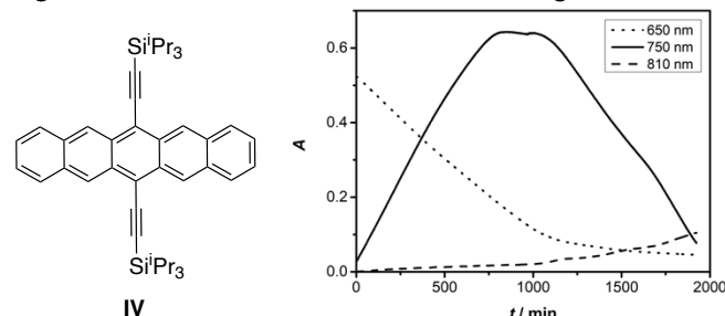
Fig. 5. Left: structure of TIPS-pentacene. Right: Evolution of absorbance at 650, 750, and 810 nm, corresponding to absorption maxima for IV , IV •- , and IV 2- , respectively, for the reaction of IV with excess 4 2b in chlorobenzene. See also Fig. S12, †ESI.
