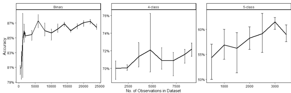
FIGURE 4 | Averaged testing accuracy as a function of number of observations used for each model. For each specified number of observations, three trials were conducted. The error bars represent the maximum and minimum errors.
