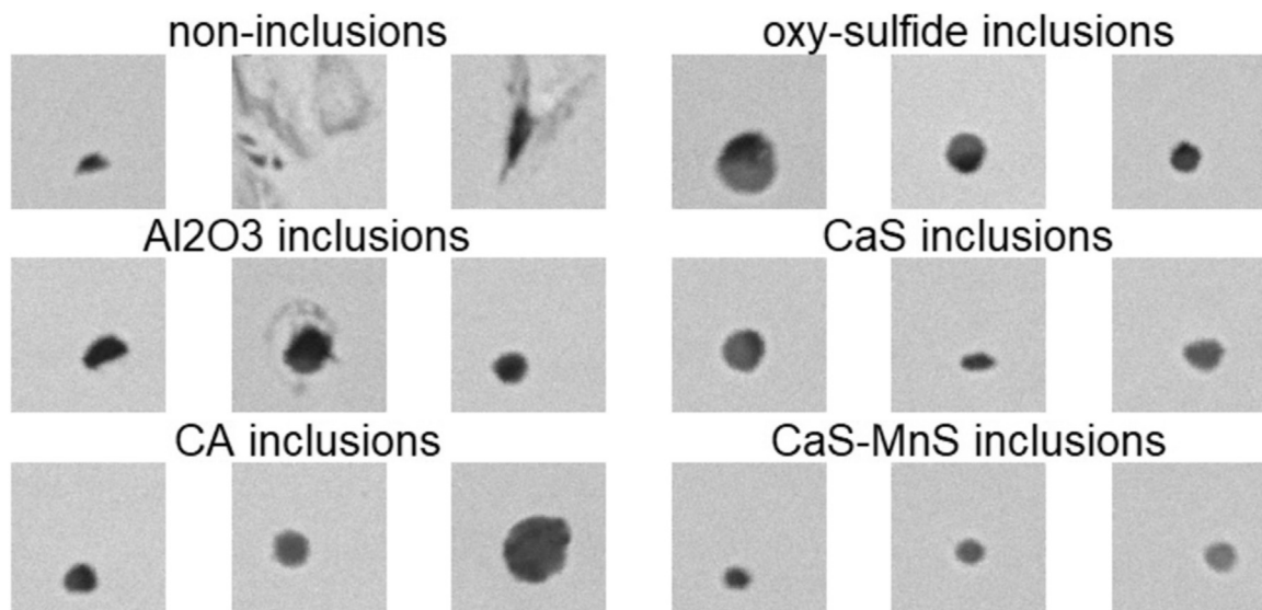
FIGURE 3 | Three BSE image examples for each of the selected inclusion classes.
