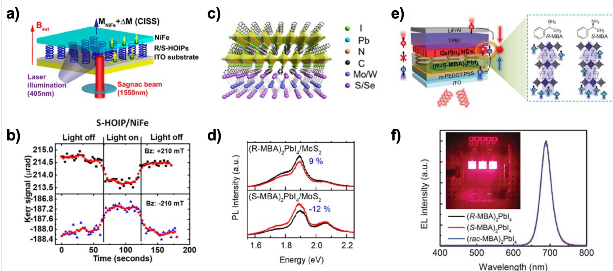
Fig. 11: (a) Schematics of the Sagnac MOKE experiment at the interface of chiral-HOIP and NiFe substrate. (b) The change in Kerr signals with photoexcitation under positive and negative out-of-plane magnetic field. 76 (c) Schematics of the chiral 2D perovskite/TMD heterostructure. (d) Polarization-resolved photoluminescence spectra of the heterostructure excited by a linearly polarized laser of 532 nm. 77 (e) Schematics of a CISS spin-LED. (f) Electroluminescence spectrum with CISS layer/CsPbI 3 heterostructures and a device image as inset. 79 Copyright 2020 by the American Chemical Society and 2021 by the American Association for the Advancement of Science.
