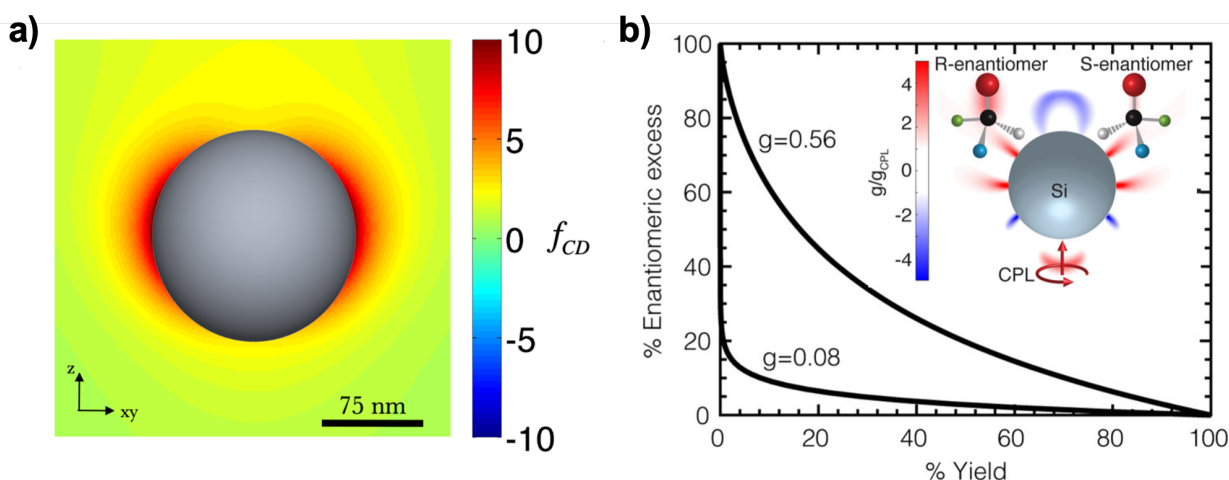
Fig. 19: (a) Nanoparticles can enhance molecular circular dichroism (CD) spectroscopy. A 75 nm radius silicon nanosphere is illuminated from below by \lambda = 625 nm circularly polarized light. The figure depicts the CD enhancement factor at a plane crossing the center of sphere. (b) When Kuhn's dissymmetry factor is increased in the vicinity of a nanoparticle, the enantiomeric excess achievable in a photochemical reaction increases dramatically for a given extent of reaction. (Inset) Spatial distribution of dissymmetry factor enhancement for a 536 nm Si sphere at \lambda = 1391.82 nm. In the presence of a Si nanosphere, in a region where g \approx 7 , a 20% enantiomeric excess can be reached with a yield of 50% compared to the 1% achievable in the absence of the nanoparticle. Panel (a) adapted from Ref. 205 with permission, copyright 2013 American Physical Society. Panel (b) adapted from Ref. 204 with permission, copyright 2017 American Chemical Society.
