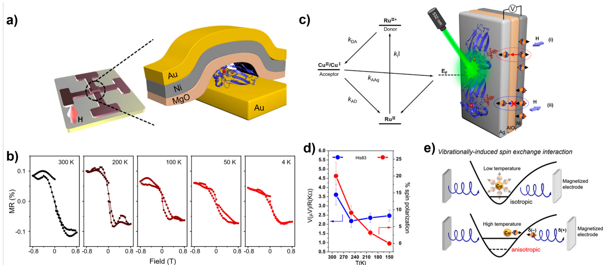
Fig. 7: Temperature dependence of spin-dependent electron transport through the protein azurin. (a) Schematic of magnetoconductance device with wild-type azurin sandwiched between ferromagnetic and normal metal electrodes. (b) Magnetoresistance measured from 300 K to 4 K. (c) Measurement scheme to detect photoinduced charge transfer between a ruthenium donor and copper acceptor groups, and a ferromagnetic substrate. (d) Spin-independent photovoltage and spin polarization percentage as a function of temperature. (e) Model of vibronically activated spin-polarization. Adapted with permission from Ref. 64. Copyright 2021 by American Chemical Society.
