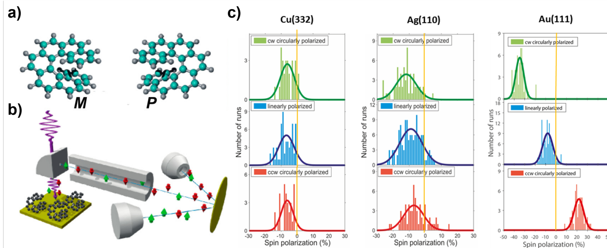
Fig. 4: Spin polarization of photoelectrons from Cu, Ag, and Au substrates transmitted through a monolayer of M hepta-helicene. (a) Structures of enantiomers. (b) Experimental setup for photoemission and Mott analyzer. (c) Green, blue, and red histograms (from top to bottom) represent excitation by clockwise (cw) circularly, linearly, and counterclockwise (ccw) circularly polarized light at \lambda = 213 nm, and thus emitting electrons slightly above the vacuum level of the systems. Adapted from Ref. 50 with permission. Copyright 2018 American Chemical Society.
