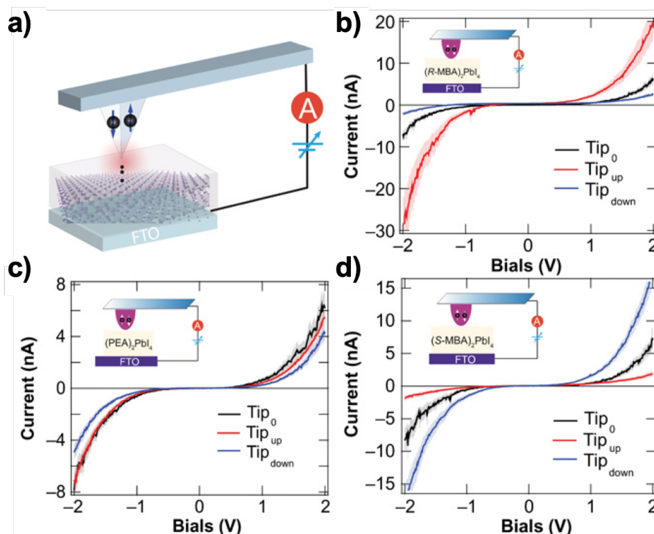
Fig. 10: (a) Experimental scheme for magnetic conductive atomic force microscopy (AFM) measurement of chiral perovskite thin films. (b)-(d) Current–voltage traces collected for thin films of lead–iodide perovskites containing chiral R-methylbenzylammonium, achiral phenylmethylamine, and chiral S-methylbenzylammonium, respectively, as a function of tip-magnetization orientation. Reproduced with permission from Ref. 73. Copyright 2019 by the American Association for the Advancement of Science.
