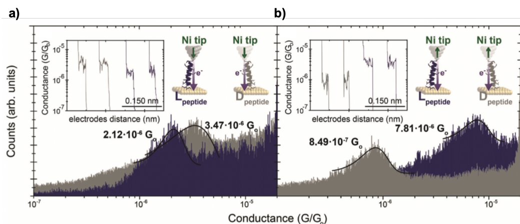
Fig. 23: Conductance histograms for hundreds of single-peptide junctions collected in different STM-BJ experiments with Ni tips magnetized a) down and b) up for both left- and right-handed alpha-helical peptides. These peptides are composed of 22 amino acid residues bridges attached to gold substrates. Insets depict representative current vs. pulling traces with well-defined single-molecule plateau features. Conductance values were extracted from Gaussian fits to the histograms. Adapted with permission from Ref. 107. Copyright 2017 by John Wiley and Sons.
