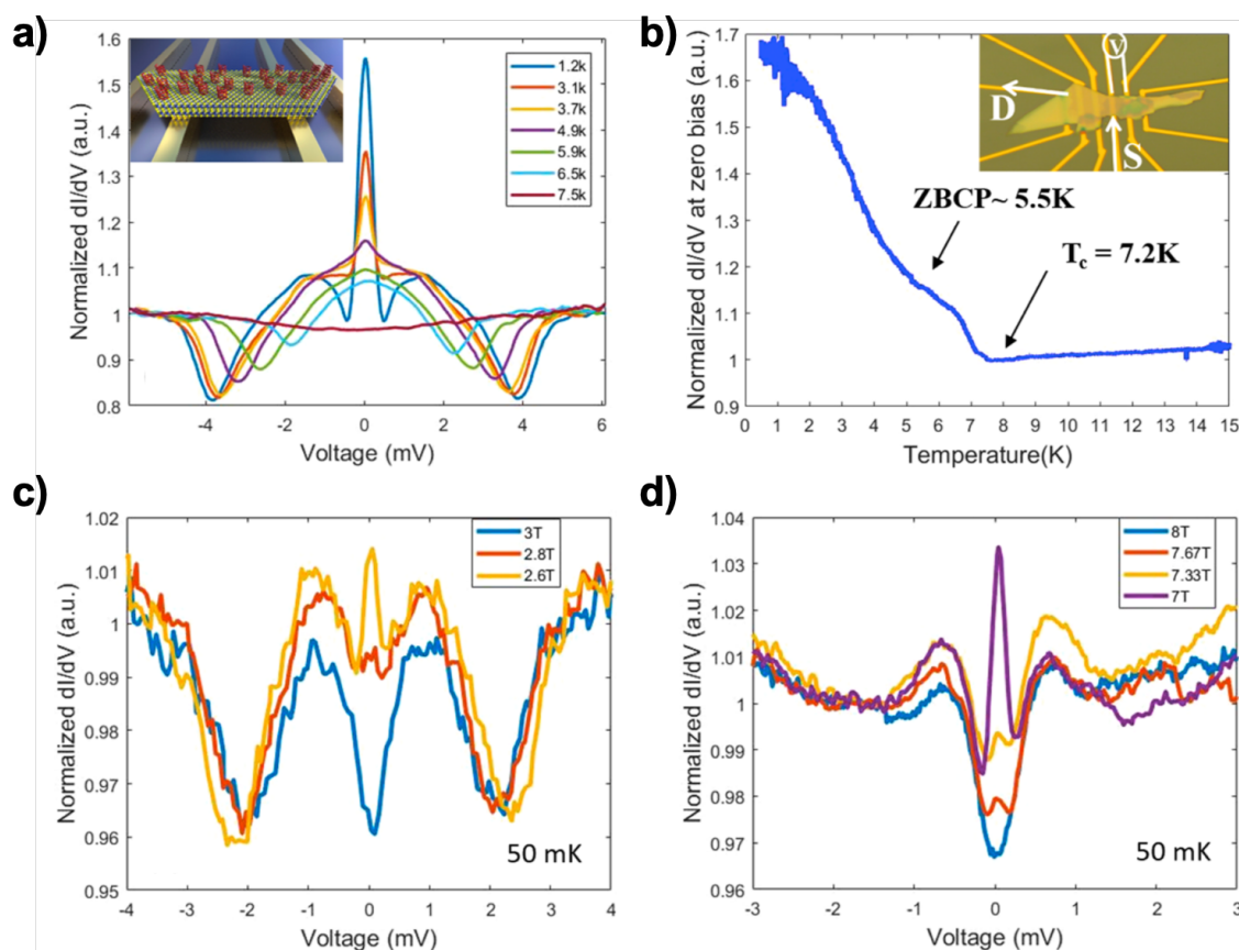
Fig. 27: Conductance properties of a low-resistance ( 120\ \Omega ) NbSe 2 /Au junction after chemisorption of chiral molecules on the NbSe 2 flake ( \sim 25 nm thick). (a) Temperature dependence of dI/dV vs. V spectra showing a distinct zero-bias conductance peak that vanishes at higher temperatures (but still below T_c ). Inset: Illustration of a chiral-molecules/NbSe 2 -flake/Au sample. (b) Temperature dependence of the conductance at zero bias with two transition temperatures marked by arrows: T_c = 7.2 K, where the zero bias conductance starts to rise due to the Andreev dome and 5.5 K where a zero bias conductance peak starts to appear. Inset: Optical image of the sample with the measurement scheme depicted. (c,d) Perpendicular (c) and parallel (d) magnetic field dependencies of the conductance spectrum, showing that in high magnetic fields, yet below the parallel and perpendicular critical fields ( H_{c2} ) of bulk NbSe 2 , the zero-bias conductance peak vanishes, revealing an underlying gap. Reproduced with permission from Ref. 339. Copyright 2019 by the American Chemical Society.
