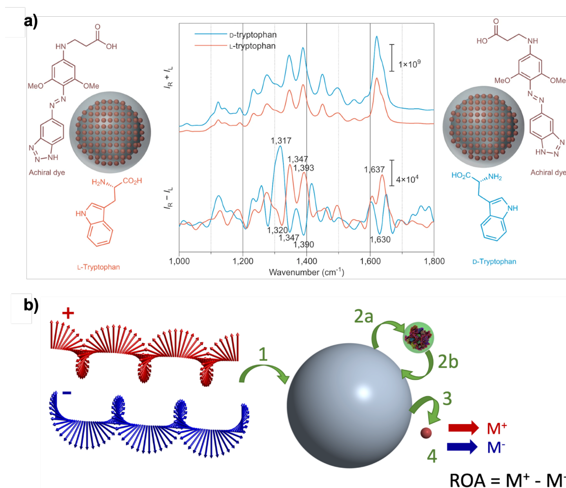
Fig. 21: (a) Schematic of the plasmonic nanoparticle–chiral molecule hybrid. The silver nanoparticle is surrounded by reporter Raman molecules, surrounded by a silica shell and has attached a chiral analyte. Middle plot shows surface enhanced resonant Raman spectra of D- and L-tryptophan bound to the benzotriazole-functionalized nanotag, which are identical as expected for the two enantiomeric systems. Surface enhanced Raman optical activity (SEROA) spectra in the presence of the two chiral enantiomers. Strong chiroptical responses in several signals are observed, demonstrating the chirality transfer phenomena. (b) Schematic of the model describing the chiral molecule–nanoparticle hybrid. Step 1: circularly polarized light excites the plasmonic nanoparticle. Steps 2a and b: The plasmonically enhanced fields excite the chiral molecule, which backscatters light into the particle, producing a self consistent chiral polarization of the plasmonic particle. Step 3: The chiral polarization of the chiral molecule–nanoparticle hybrid excites the non-chiral Raman reporter. Step 4: The Raman molecule emits a surface enhanced resonant Raman signal, which is different for left handed ( M^+ ) and right handed ( M^- ) circularly polarized incidence, creating a measurable Raman optical activity signal. Panel (a) Reprinted and adapted with permission from Ref. 17 based on work in Ref. 224, copyright 2015 Nature Publishing Group. Panel (b) adapted with permission from Ref. 225, copyright 2020 American Chemical Society.
