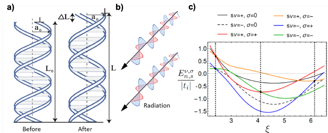
Fig. 30: Effects of light on chiral molecules through the Floquet approach to achieve stretch and spectral engineering. (a) Molecules can be made to stretch or contract by impinging light (b) modulating the SO coupling (modified figure from Ref. 137). (c) Spectrum normalized by base pair to base pair overlap strength as a function of spin state ( s ), transport direction ( \nu ) and pseudo-spin quantum ( \sigma ) vs. the normalized frequency ( \xi ) of impinging light.
