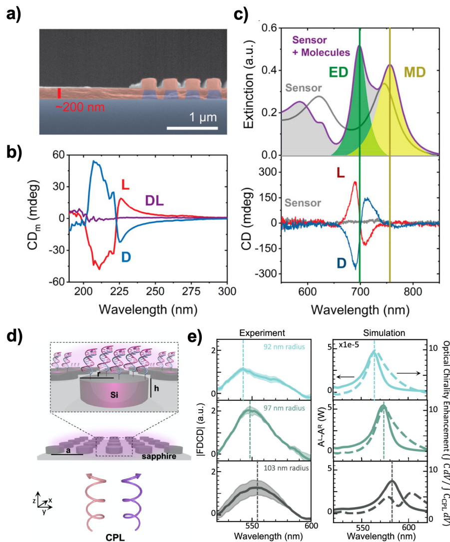
Fig. 20: (a) Scanning electron micrograph of a Si nanodisk array coated with a ca. 200 nm phenylalanine layer. (b,c) Experimentally measured circular dichroism and extinction spectra of Si nanodisk sensor arrays functionalized with phenylalanine coatings. Panels (a)-(c) adapted from Ref. 211 with permission. Copyright 2019 American Chemical Society. (d) Experimental schematic of fluorescence-detected circular dichroism (FDCD) using Si nanodisk arrays modified with self-assembled monolayers of chromophore-functionalized DNA molecules. (e) Experimentally measured FDCD and enhancement in optical chirality density for increasing disk sizes when functionalized with DNA monolayers. Panels (d)-(e) adapted from Ref. 217 with permission. Copyright 2020 American Chemical Society.
