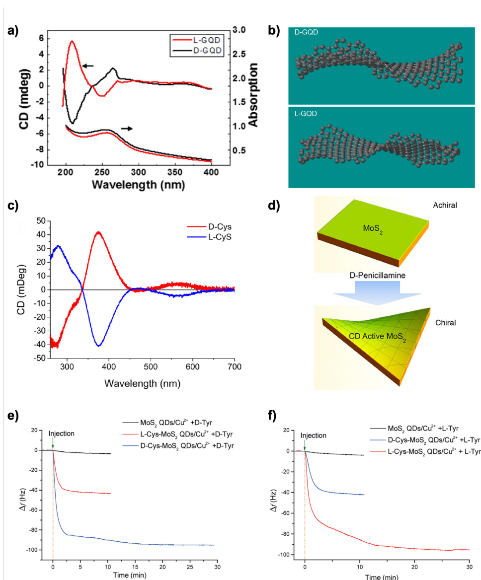
Fig. 22: (a) Circular dichroism (CD) and optical absorption spectra for L-graphene quantum dots (L-GQD) (red) and D-GQD (black) dispersions. (b) Schematic of the structures of D-GQD and L-GQD on a 3 nm QD. The rotation direction of the helices is opposite to the handedness of the edge-ligands. (c) Circular dichroism spectra of D/L-cysteine functionalized MoS 2 after exfoliation. Similar results for D-/L-penicillamine were obtained (not shown here). (d) Diagram of the deformations generated by molecular functionalization of D-penicillamine inducing chirality on MoS 2 layers. (e–f) Frequency shifts of the D- and L-Cys–MoS 2 QDs/Cu 2+ sensors exposed to (e) 5 mM D-Tyr and (f) 5 mM L-Tyr solution. Panels (a)–(b) adapted with permission from Ref. 227. Copyright 2016 by the American Chemical Society. Panels (c)–(d) adapted with permission from Ref. 235. Copyright 2018 by the American Chemical Society. Panels (e)–(f) adapted from Ref. 248 with permission. Copyright 2018 by the American Chemical Society.
