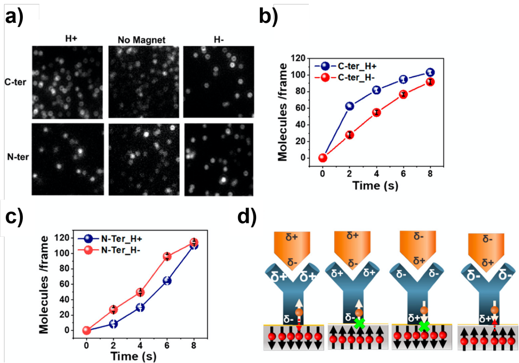
Fig. 8: Evidence for allosteric long-range charge reorganization in proteins. (a) Fluorescence microscopy images of antibody-antigen binding to oppositely magnetized substrates. (b,c) Reaction kinetics of the binding interaction. (d) Schematic of the spin-valve like behavior gating charge reorganization when antibodies are adsorbed on ferromagnetic substrates. Reproduced with permission from Ref. 67. Copyright 2020 by American Chemical Society.
