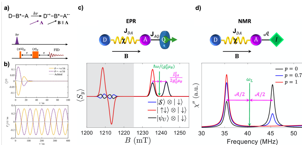
Fig. 25: (a) Schematic of radical pair formation in donor–bridge–acceptor species and pulse sequence in a hypothetical out of phase electron spin echo envelope modulation (OOP-ESEEM) EPR experiment. (b) Calculated OOP-ESEEM signal from opposite enantiomers in a chiral radical pairs showing different phase shifts. Adapted with permission from Ref. 329. (c) Proposed EPR and (d) NMR experiments to elucidate the role of chiral linkers in spin-dependent transfer in chiral donor–bridge–acceptor pairs. Copyright 2021 by American Chemical Society. Adapted with permission from Ref. 330. Copyright 2021 by American Chemical Society.
