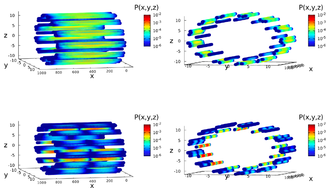
Fig. 32: The quantum probability of finding the collective excitonic state on a single tryptophan residue of a microtubule segment is shown for an extended superradiant state (top row) and subradiant state (bottom row) in lateral view (left column) and in cross section (right column). Microtubule segment consists of 100 spirals (greater than 800 nm) with 10,400 tryptophan residues. Reproduced with permission from Ref. 406. Copyright 2019 by IOP Publishing Ltd.
