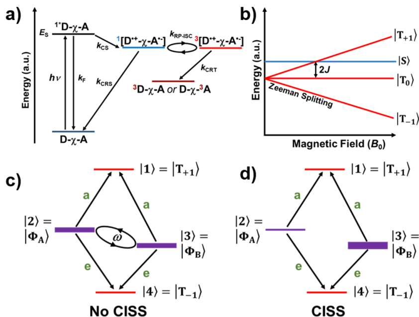
Fig. 24: (a) Electron transfer and intersystem crossing pathways in a (D-\chi-A) system, where k_{CS} is the charge separation rate constant, k_{RP-ISC} is the radical pair intersystem crossing rate constant, and k_{CRS} and k_{CRT} are the charge recombination rates via the singlet and triplet channels, respectively. (b) (D^+ - \chi - A^-) energy levels as a function of magnetic field for 2J > 0 , D = 0 . (c) (D^+ - \chi - A^-) energy levels in the high field limit with no CISS, where \omega is the mixing frequency and the enhanced absorptive ( a ) and emissive ( e ) microwave-induced transitions are indicated. (d) (D^+ - \chi - A^-) energy levels with CISS in which only |3\rangle is populated.
