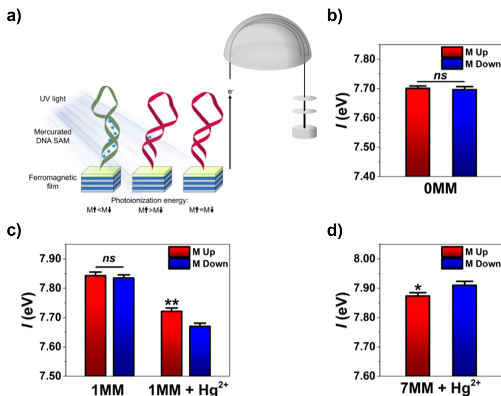
Fig. 3: Spin-dependent photoelectron scattering of DNA hairpins. (a) Schematic depicting spin-dependent photoelectron scattering through self-assembled monolayers of DNA hairpins on ferromagnetic films, characterized by ultraviolet photoelectron spectroscopy. Spin-dependent ionization cross sections result in differential charging, physically manifested as substrate magnetization-dependent photoionization energies of the chiral organic films. (b,c) Spin-selective effects were only observed in short ( \sim 1 helical turn) DNA hairpins that contained mercury bound at thymine–thymine mismatches due to enhanced molecular SO coupling. (d) Spin selectivity was reversed in DNA hairpins containing 7 mismatches and stoichiometric amounts of mercury ions, which was shown to invert the chirality of the helical hairpins. Reproduced with permission from Ref. 47. Copyright 2020 by the American Chemical Society.
