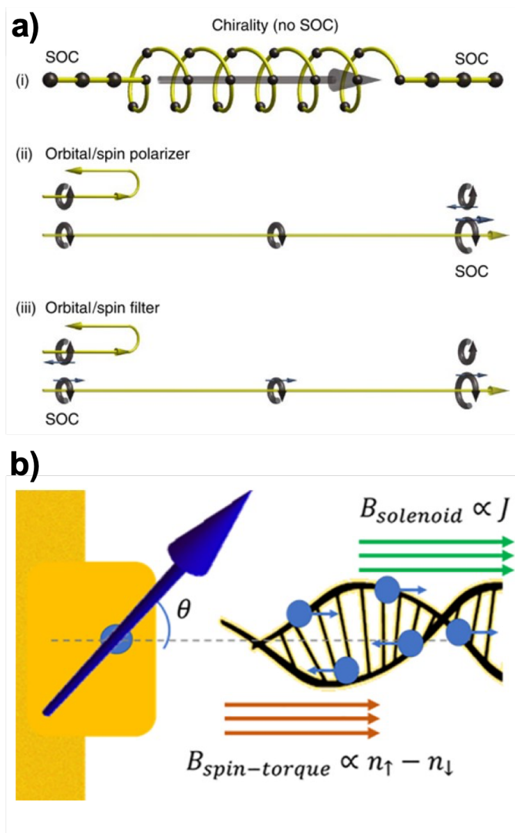
Fig. 16: (a) Schematics of the orbital polarization effect. (i) A chiral molecule is connected to two leads on each end and (ii) acts as both an orbital polarizer and (iii) an orbital filter. The half circles with arrows represent the orbital and thin arrows represent the spin. 130 (b) Schematics of the description of the origin of CISS effect. The interface orbital magnetization is indicated by the blue arrow at a tilted angle. It interacts with two effective magnetic fields: the solenoid field and the spin-torque field. 131 Images reproduced with permissions. Copyright 2021 by Springer Nature and the American Chemistry Society.
