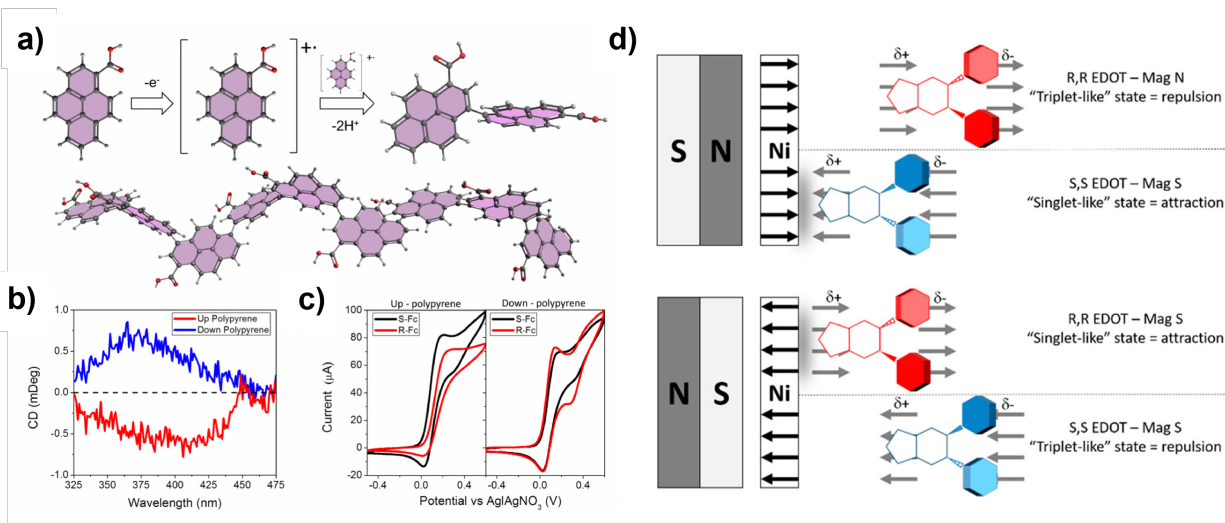
Fig. 9: Reaction scheme and chirality in electropolymerization. (a) Reaction scheme for the polymerization of 1-pyrenecarboxylic acids into polypyrene which exhibits a helical twist (see main text for more details). (b) Circular dichroism spectra for electrodes coated with polypyrene where a magnetic field was applied Up (red) or Down (blue) during electropolymerization. (c) Electrochemistry measurements on (S)- (black) or (R)-ferrocene (red) with the Up (left) or Down (right) polypyrene-coated working electrodes. Reproduced with permission from Ref. 69. Copyright 2020 by John Wiley and Sons. (d) Interaction scheme between a ferromagnetic electrode and chiral monomers. Reproduced with permission from Ref. 70. Copyright 2020 by American Chemical Society.
