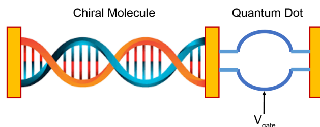
Fig. 28: A schematic illustration of a ‘super chiral molecule’ – a coupled chiral-molecule/quantum-dot hybrid structure, for controlling and manipulating spin polarization and entanglement. The gate voltage is applied to change the QD structure for controlling spin polarization.
