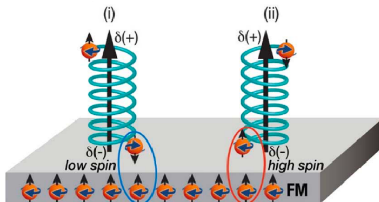
Fig. 6: Interactions between chiral molecules and ferromagnetic surfaces. As a chiral molecule approaches the ferromagnetic (FM) substrate, its charge polarization generates a spin polarization at the two ends of the molecule. For a specific enantiomer, the interaction between the magnetized surface and the molecule (circled in blue and red) follows a low-spin or a high-spin potential, depending on the direction of magnetization of the substrate. Reproduced with permission from Ref. 57. Copyright 2018 by The American Association for the Advancement of Science.
