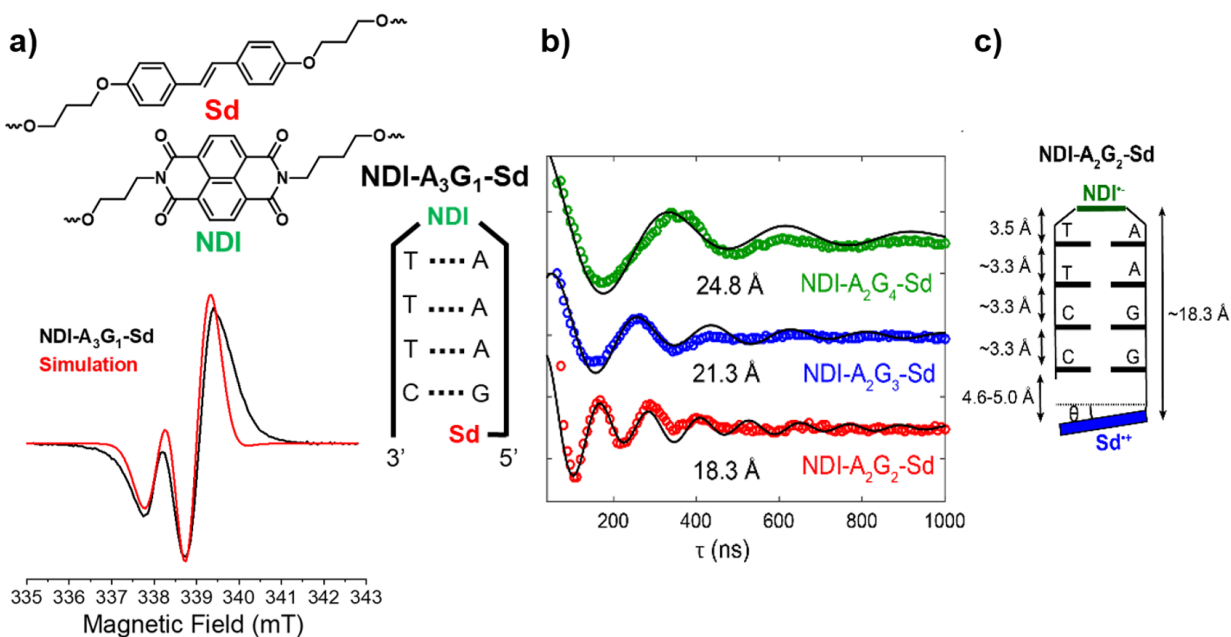
Fig. 26: (a) Time-resolved electron paramagnetic resonance spectrum of NDI - A_3G_1 - Sd at 85 K, 100 ns after a 355 nm, 7 ns laser pulse (black trace) and its simulation (red trace). (b) OOP-ESEEM for NDI - A_2G_n - Sd hairpins. Experimental data are shown for NDI - A_2G_2 - Sd (red), NDI - A_2G_3 - Sd (blue), and NDI - A_2G_4 - Sd (green). Simulated echo modulations (black) used to predict the SCRPs distances listed for each hairpin based on the extracted dipolar coupling constant. (c) Cartoon of NDI - A_2G_2 - Sd illustrating the rotation of the Sd end cap necessary to achieve the measured radical pair distances between NDI^- and Sd^+ . Copyright 2019 by American Chemical Society. Adapted with permission from Ref. 318.
