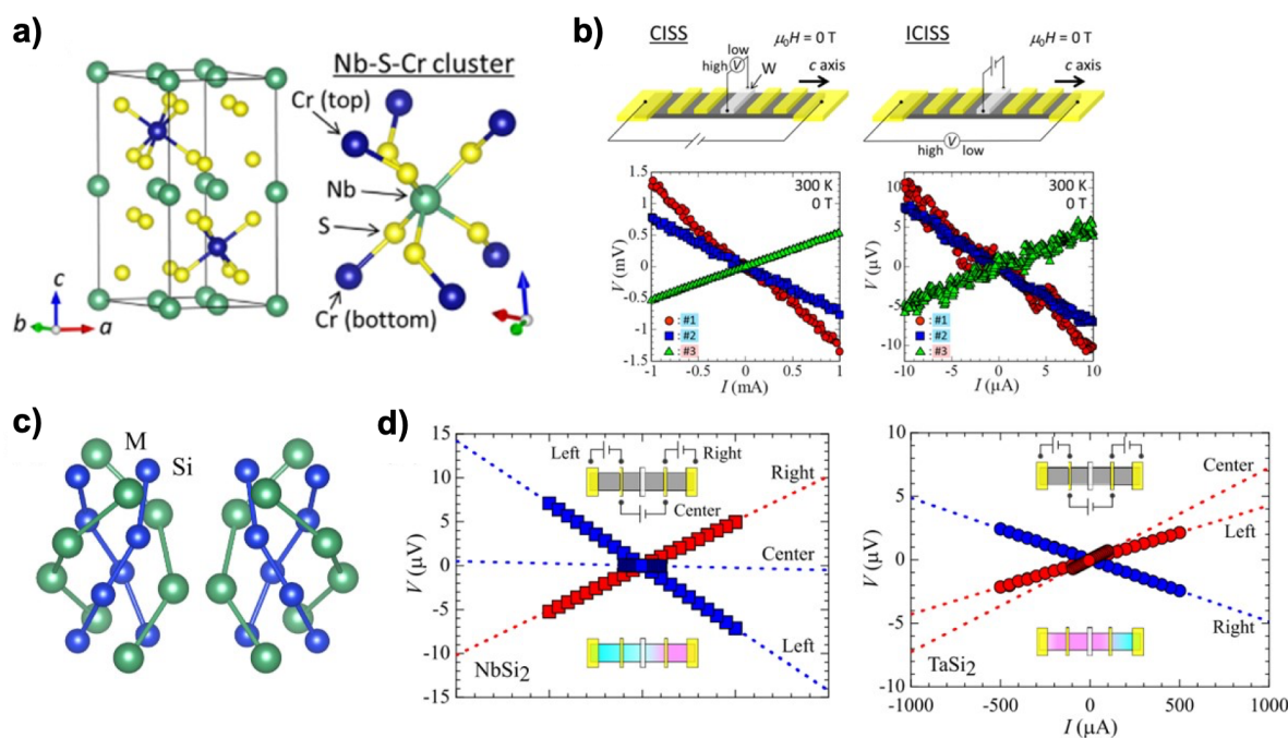
Fig. 12: (a) Schematics of crystal structures of CrNb 3 S 6 . (b) Schematics and electrical measurements of CISS and inverse CISS signals. 80 (c) Schematics of crystal structures of a disilicide compound MSi 2 (M: transition metal). (d) Location variations of the CISS signals of NbSi 2 and TaSi 2 . 81 Reproduced with permissions from Refs. 80,81. Copyright 2020 and 2021 by the American Physics Society.
