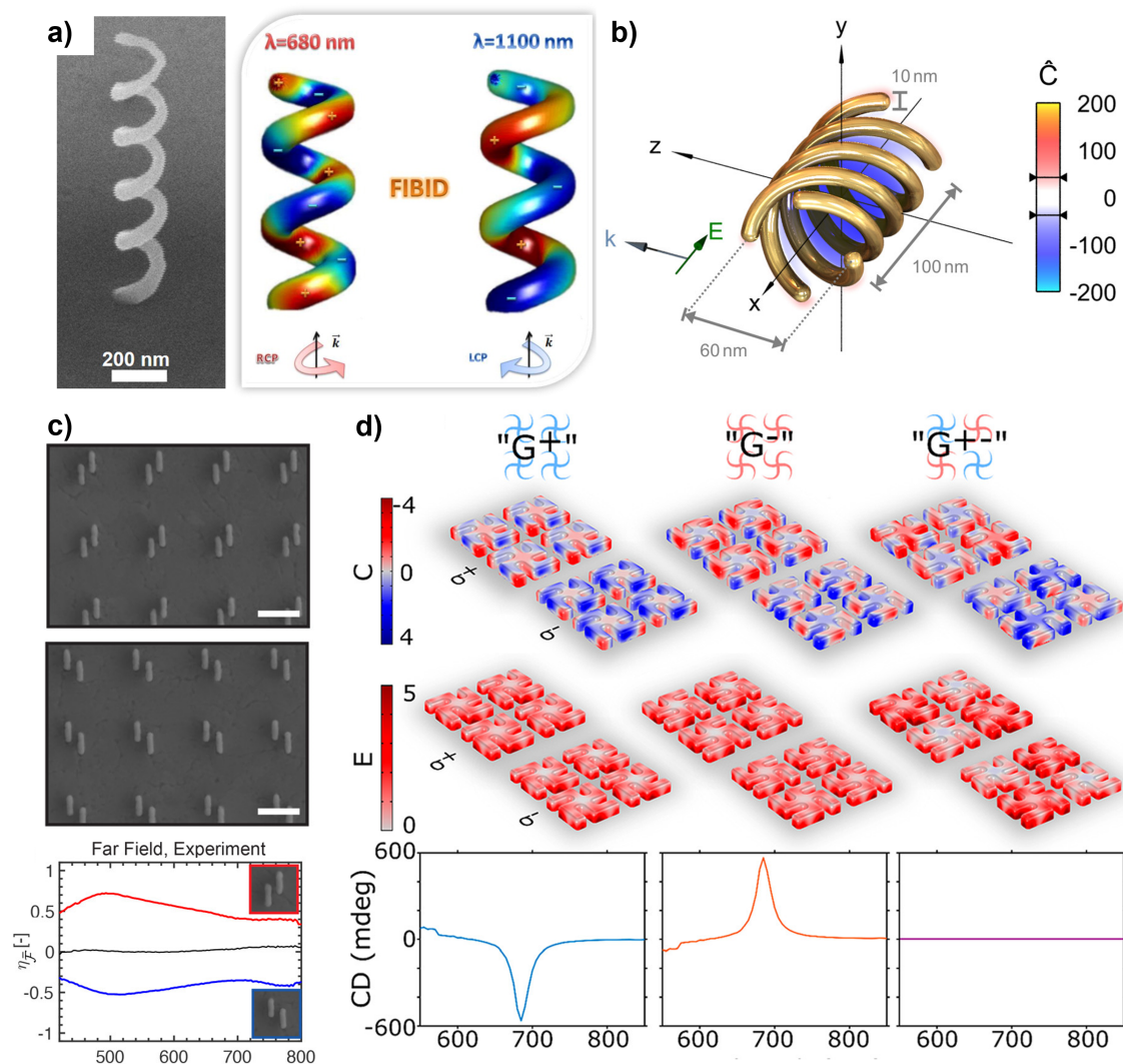
Fig. 18: (a) Scanning electron microscope (SEM) image of a platinum chiral nanohelix grown by focused ion beam induced deposition (FIBID) and a three-dimensional representation of current oscillation induced by exciting on resonance for the right- and left-handed resonance modes. 183 Copyright 2015 by the American Chemical Society. (b) Strongly enhanced optical chirality density (C) theoretically predicted to be generated within plasmonic helices. 170 Copyright 2015 by the American Chemical Society. (c) SEM images of left- and right-handed planar chiral coupled nanorod antennas and experimentally measured chirality flux efficiency for each configuration. 178 Copyright 2018 by the American Chemical Society. (d) Optical chirality density enhancement, electric field enhancement, and circular dichroism calculated for ure left- and right-handed as well as racemic mixtures of plasmonic gammadion arrays. 181 Copyright 2018 by the American Chemical Society.
