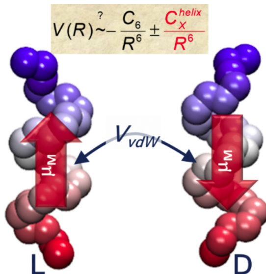
Fig. 14: In the case of chiral molecules, induction and dispersion forces encoding electric dipole-dipole interactions require additional modifications to account for exchange-mediated interactions related to the CISS effect.
