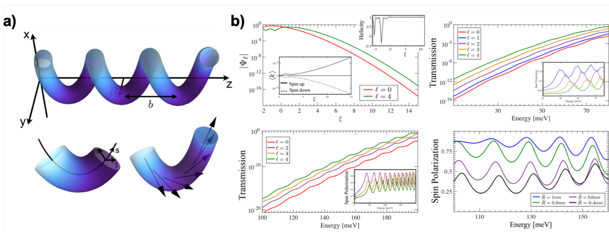
Fig. 15: (a) The helical tube. Electrons are confined to a helical tube of radius R and pitch b . s is the position along the helix tube and vectors n and t span the plane perpendicular to s . A term in the Hamiltonian acts as an effective Zeeman field rotating as a function of the position along the helix. Adapted with permission from Ref. 127. (b) Transmission through an helix-shaped molecule in the presence of a dipole field. (Top left) In the presence of SO coupling, the amplitude of the (exact) electronic wave function in its tail (parametrized by \xi \gg 1 ) grows as a function of the angular momentum. Moreover, the spin is aligned along the momentum direction (see inset), and as a consequence the state has a well defined helicity. (Top right) The increased amplitude deep inside the molecule gives rise to an enhanced transmission probability that grows with the angular momentum \ell . The scattering matrix 128 is derived for the exact wave function. This panel shows that the enhanced transmission for \ell \neq 0 is accompanied by a spin polarization (inset). (Bottom left) Similar results were obtained using a tight binding calculation for a molecule with the same parameter but somewhat different length. (Bottom right) Deforming the molecule to have a larger pitch or radius helps spin polarization. Adapted with permission from Ref. 127. Copyright 2020 American Chemical Society.
