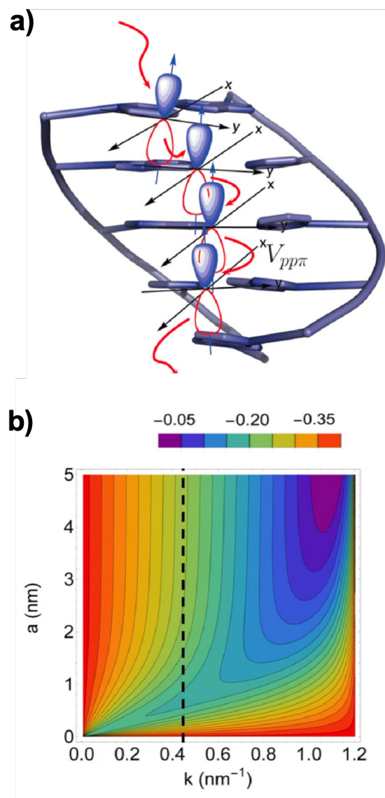
Fig. 17: Spin-orbit interactions and spin selectivity for tunneling electron transfer in DNA. (a) Schematic of DNA molecule with orbitals for electron transport. The p_z orbitals are perpendicular to the base planes and coupled by V_{pp\pi} Slater-Koster matrix elements. (b) Plot of spin asymmetry P_z as a function of scattering barrier length a and input momentum k . Adapted with permission from Ref. 141. Copyright 2020 by the American Physical Society.
