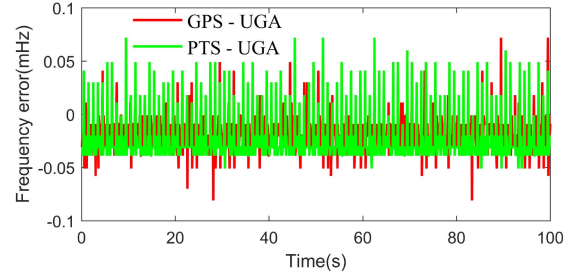
Fig. 4. Frequency error of GPS-UGA and PTS-UGA.
