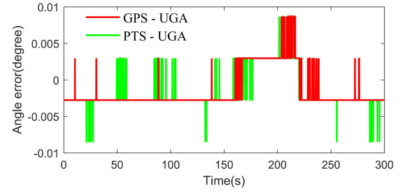
Fig. 3. Angle error of GPS-UGA and PTS-UGA.
