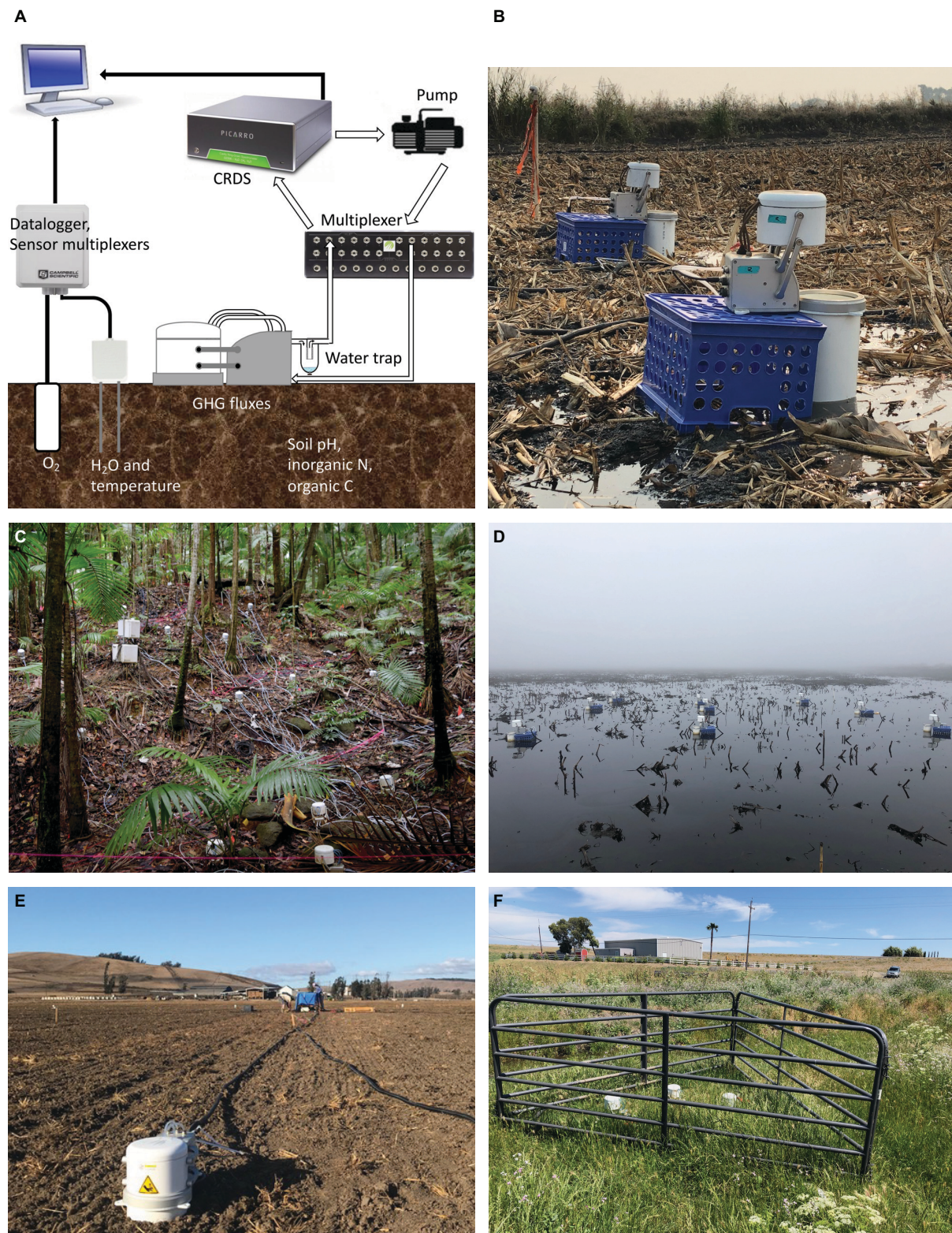
FIGURE 1 | (A) Sampling configuration for continuous soil GHG emissions by CRDS and applicable soil physicochemical variables (in this case, e.g., soil moisture, temperature, and oxygen sensors). A circulating pump draws air after chamber enclosure. The air passes through a multiplexer where is directed to the CRDS for pseudo-continuous GHG concentration measurements. (B–F) Field deployment of automated CRDS systems including in tropical high-rainfall ecosystem [Luquillo Experimental Forest, Puerto Rico (C) ], in flooded soils [California, United States (B,D) ] and agricultural systems [California, United States (E,F) ].
