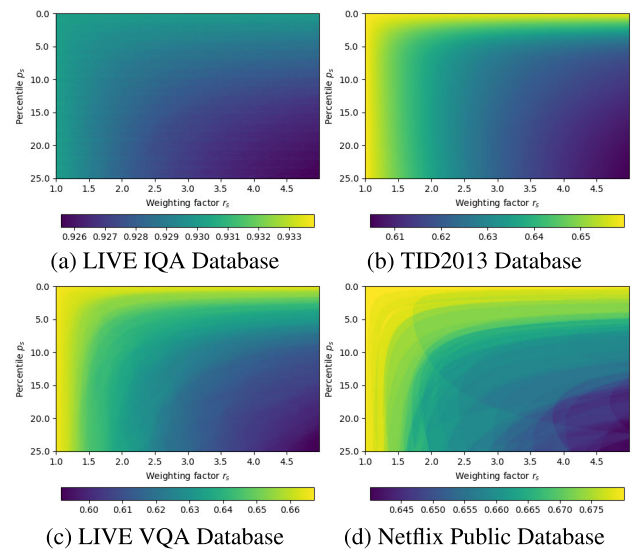
FIGURE 12. Spatial PP SROCC vs parameters p_s and r_s .
