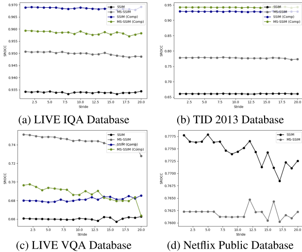
FIGURE 8. Variation of performance with stride.
