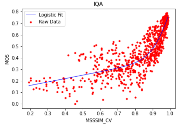
FIGURE 9. Example of fitting SPL curve to a scatter plot of MOS vs. MS-SSIM.
