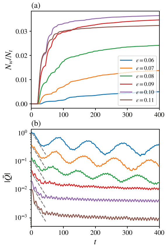
FIG. 7. Simulation of the time evolution of an initially flat-top vortex in the region of strains \varepsilon = 0.06 – 0.11 in which vortex elements (fluid particles) cross the separatrix. (a) the number of particles hitting the wall N_w is normalized by the total number of particles N_t . (b) Time dependence of the quadrupole moment normalized by Q(t_h) with the plots shifted vertically for visibility. The initial decay corresponds to that of the unstrained case [BDL Eq. (9), dash lines]. See text for details.
