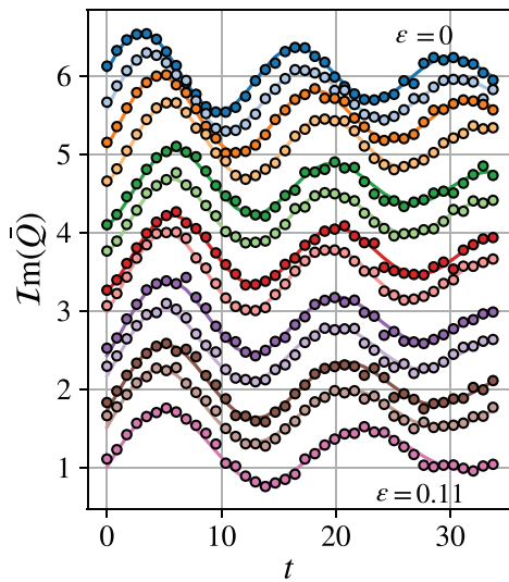
FIG. 4. Evolution of the quadrupole moment normalized by its initial amplitude and shifted vertically for visibility for strain values \varepsilon = 0 - 0.11 . The top curve is the free case ( \varepsilon = 0 ), and the bottom curve is the highest strain value, \varepsilon = 0.11 . The solid lines are fits the data using Eq. (14).
