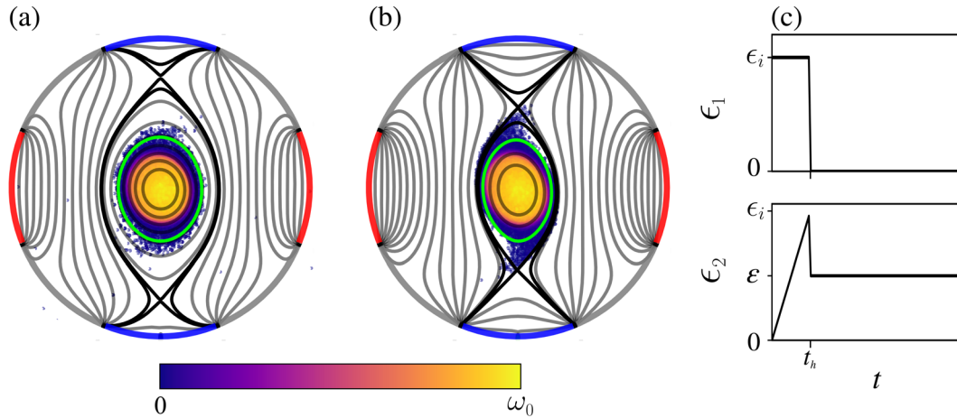
FIG. 1. (a) and (b) Cross section of the electron plasma with applied non-rotating strain boundary +V (red) and -V (blue). The strains applied are (a) \epsilon = 0.036 and (b) \epsilon = 0.073 . The first resonant layers are indicated with green lines and the separatrices with black lines. (c) Two time-dependent strain protocols: a square pulse ( \epsilon_1 ) and a linear ramp and hold ( \epsilon_2 ).
