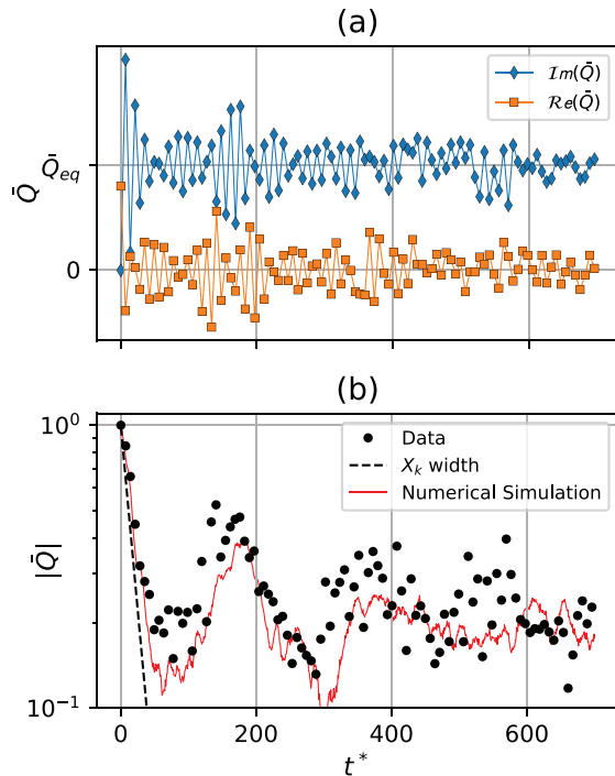
FIG. 6. (a) The two components of the quadrupole moment oscillating over \sim 50 rotations for \varepsilon = 0.025 ; and (b) the relative quadrupole moment from the equilibrium compared with numerical simulation data at the same strain rate. The solid line in (a) connects the data points as a guide for the eye.
