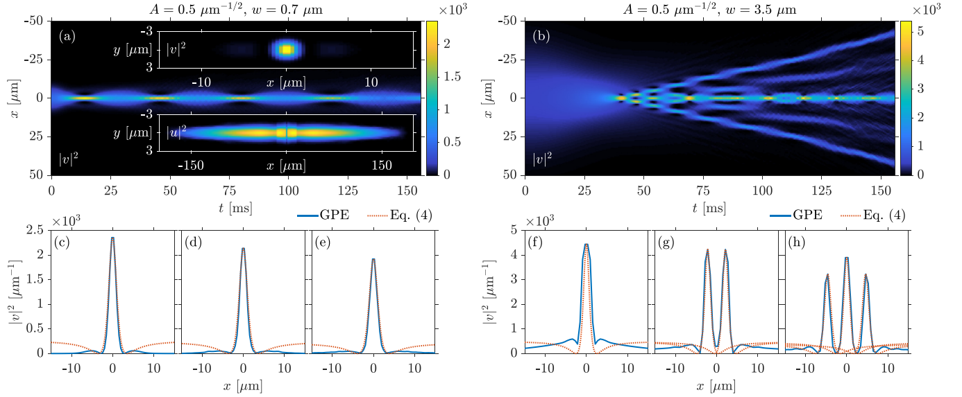
FIG. 7. (a) [(b)] Spatiotemporal evolution of the integrated along the yz direction density, of the minority v component for A = 0.5 \mu\text{m}^{-1/2} and w = 0.7 \mu\text{m} [ w = 3.5 \mu\text{m} ]. Insets in panel (a) depict density snapshots of the (top) v and (bottom) u components, rescaled by a factor of 1/3 and 1/7 , respectively, in the x - y plane at t_0 \approx 13.5 ms when the Peregrine initially forms. Panels (c)–(e) [(f)–(h)]: Integrated density profiles at selective time instants during evolution of the Peregrine and its revivals [of the Christmas tree]. A comparison with the relevant analytical prediction of Eq. (4) is also provided (see legends). For this quasi-1D evolution, the corresponding trapping frequencies are (\omega_x, \omega_y, \omega_z) = 2\pi \times (3.06, 400, 400) Hz and N = 7 \times 10^5 .
