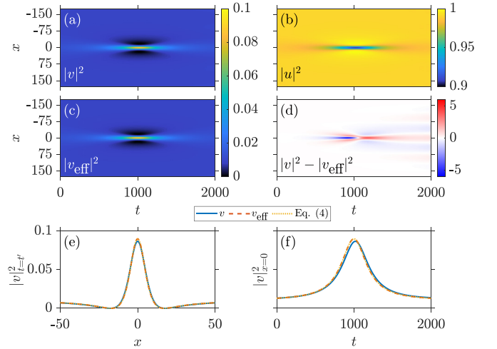
FIG. 1. Density evolution of the Peregrine initial condition [Eq. (4)] in the absence of a trap for (a) the minority and (b) the majority species of the two-component setting with \mu_u = 1 . Equation (4) is initialized with P_o = 0.01 and t_o = 1000 . (c) Dynamics of the density within the effective single-component model. (d) Density difference between the (a) two- and the (c) single-component dynamics (the color bar is rescaled by a factor of 10^3 ). (e) Density profile of the v component for the two- and single-component setups at the time instant of Peregrine formation, namely t'_{\text{two}} = 1019 and t'_{\text{single}} = 1000 . (f) Temporal evolution of the Peregrine wave emerging in the v component of both the two- and single-component setups at x = 0 (see legend). In both panels (e) and (f), the corresponding analytical Peregrine solution of Eq. (4) is provided. Note that length and time are measured in units of a_{\perp} and \omega_{\perp}^{-1} , respectively.
