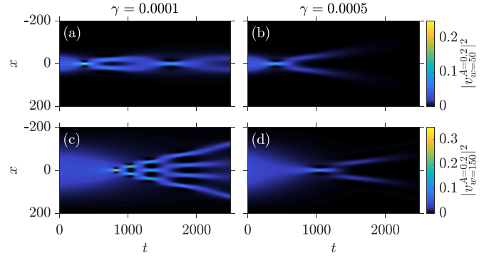
FIG. 6. Dynamical evolution of the density of the minority v component for A = 0.2 and [(a), (b)] w = 50 and [(c), (d)] w = 150 . The dissipation strength is [(a), (c)] \gamma = 10^{-4} and [(b), (d)] \gamma = 5 \times 10^{-4} . Other parameters used are \mu_u = 1 , \mu_v = 0.01 , m_u = m_v , and \Omega = 0.002 . Note that length (time) is in units of a_\perp ( \omega_\perp^{-1} ).
