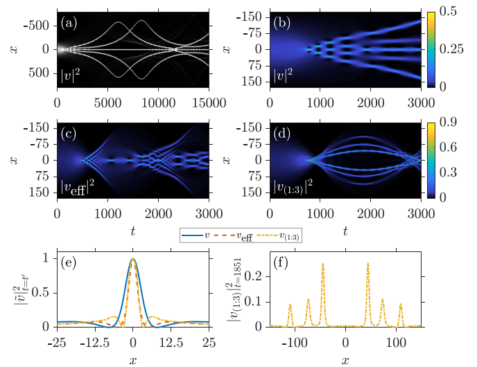
FIG. 5. Evolution of the density of a Gaussian wave packet with A = 0.2 and w = 150 in the presence of a harmonic trap with \Omega = 0.002 . (a) Temporal evolution of the minority v component. (b) A magnification of (a) is provided. (c) Effective single-component case. (d) Same as (b) but upon considering a mass-imbalanced BEC mixture (see text). (e) Density profiles of the v component for the single-component and mass-balanced and mass-imbalanced two-component setups at the instant of formation of the Peregrine soliton t'_{\text{single}} = 516 , t'_{\text{two}} = 800 , and t'_{(1:3)} = 795 , respectively. All Peregrine amplitudes are normalized to unity for direct comparison. (f) Density profile at t'_{(1:3)} = 1851 , depicting the pairwise DB soliton nucleation that follows the decay of the Christmas-tree pattern, for the mass-imbalanced mixture. In all cases, the majority u component complements its relevant minority one, and thus it is omitted. The length and time units shown are in terms of a_{\perp} and \omega_{\perp}^{-1} , respectively.
