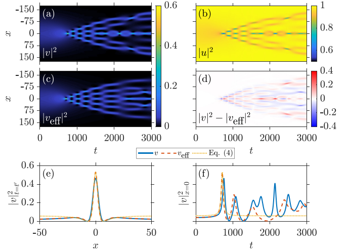
FIG. 4. Same as Fig. 3 but considering a significantly broader Gaussian initial condition with w = 150 . In this case, the Peregrine soliton formation within the two models occurs at t'_{\text{two}} = 758 and t'_{\text{single}} = 716 , respectively. Notice also the subsequent emergence of the Christmas-tree structure. Recall that length and time are given in units of a_{\perp} and \omega_{\perp}^{-1} , respectively.
