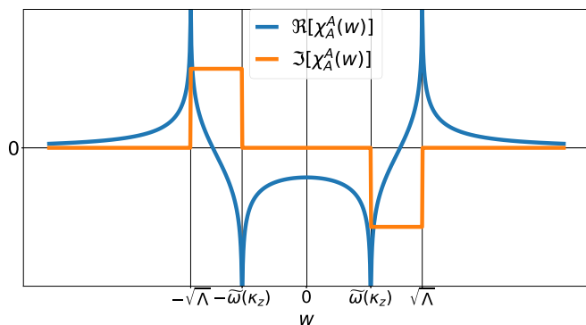
FIG. 17. Real \Re[\chi_A^A(w)] and imaginary \Im[\chi_A^A(w)] parts of the A-field response function \chi_A^A(w) in the effective field theory with \eta = 0 . The imaginary part has a finite value within the frequency window \tilde{\omega}(\kappa_z) < |w| < \sqrt{\Lambda} which indicates that in this frequency range the system can continuously absorb energy. The real part though diverges at the natural lower cutoff w = \pm\tilde{\omega}(\kappa_z) and the upper cutoff w = \pm\sqrt{\Lambda} and shows that the system in the effective field theory has two scales.
