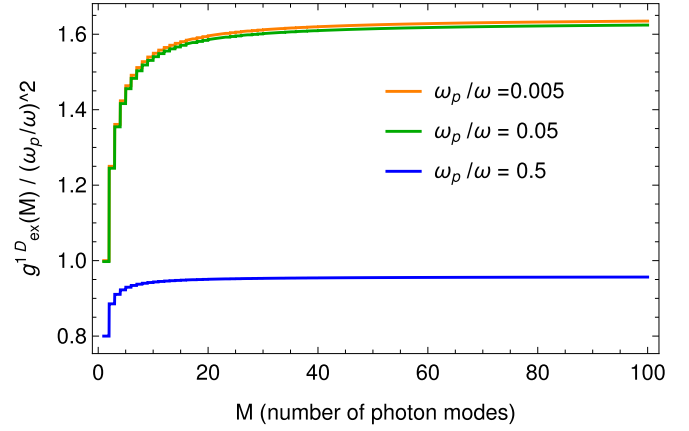
FIG. 13. Exact many-mode coupling constant g_{\text{ex}}^{1D}(M) normalized by (\omega_p/\omega)^2 in 1D, as a function of the number of photon modes M . The exact coupling is plotted for three different values of the ratio \omega_p/\omega corresponding to different regimes of light-matter interaction. In all cases we see that the exact coupling has arctangent dependence on the amount of photon modes. The exact coupling is normalized by (\omega_p/\omega)^2 such that all graphs to be visible in one plot.
