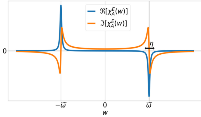
FIG. 7. Real \Re[\chi_A^E(w)] and imaginary \Im[\chi_A^E(w)] parts of the E-field response function \chi_A^E(w) in the frequency domain with a finite broadening parameter \eta . The poles of \Re[\chi_A^E(w)] and \Im[\chi_A^E(w)] both appear at the frequency w = \pm\tilde{\omega} and signify the frequency at which an time-dependent electric field is oscillating. Radiation should come out of the cavity at this frequency.
