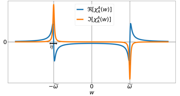
FIG. 6. Real \Re[\chi_A^A(w)] and imaginary \Im[\chi_A^A(w)] parts of the \mathbf{A} -field response function \chi_A^A(w) in the frequency domain, plotted with a finite \eta . The resonances for both parts appear at the plasmon-polariton frequency w = \pm\tilde{\omega} .
