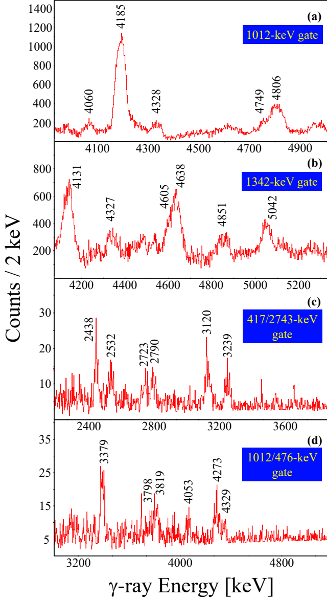
FIG. 1: (Color online) (a) \gamma - \gamma coincidence spectrum with a gate placed on the 1012-keV transition from the 2^+ , 2069-keV level in ^{26}\text{Al} . (b) \gamma - \gamma coincidence spectrum with a gate placed on the 1342-keV transition from the 2^+ , 1759-keV level in ^{26}\text{Al} . (c) \gamma - \gamma - \gamma spectrum with gates placed on the 2743- and 417-keV transitions showing coincidences with the 2^+ , 3160-keV level in ^{26}\text{Al} . (d) \gamma - \gamma - \gamma spectrum with gates placed on the 476- and 1012-keV transitions showing coincidences with the 3^+ , 2545-keV level in ^{26}\text{Al} .
