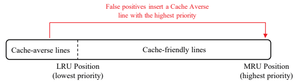
Figure 17: A costly binary classification error in Hawkeye.
