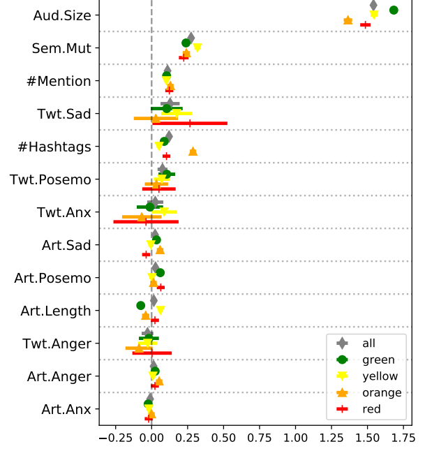
Figure 3: Logistic Regression Coefficients with 95% confidence interval. In each sub-figure, the variables are sorted by the estimated coefficients of the all sub-dataset. The coefficients of the topic variables are omitted in the figure for readability. (a) Variable Coefficients of the Originality Predicting the Popularity in Logistic Regression. Among all variables besides the audience size, the Originality has the highest coefficient values in most data subsets (except for the Red set, where the estimated coefficient value of sadness in comment (Twt.Sad) is greater). (b) Variable Coefficients of the Sem.Mut Predicting the Popularity. The Sem.Mut have greater estimated coefficients than most of the other variables including the emotional cues in article texts and emotional cues in the users' comments (except for sadness).
