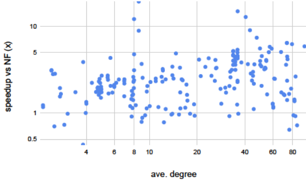
Figure 8. Speedup of ADDS over NF vs. graph degree.
