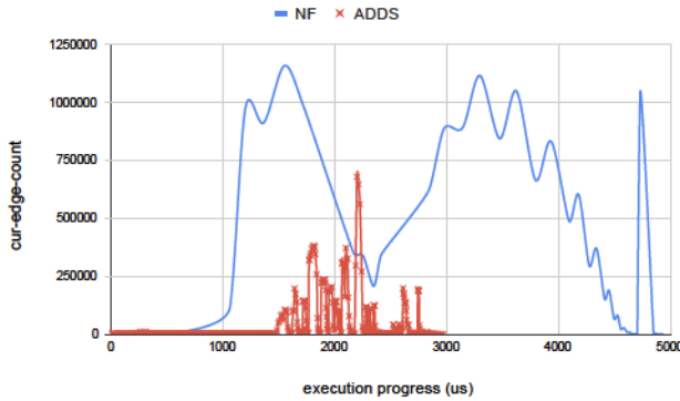
Figure 15. E.c-big: s:1.6×, w:3.35×.
