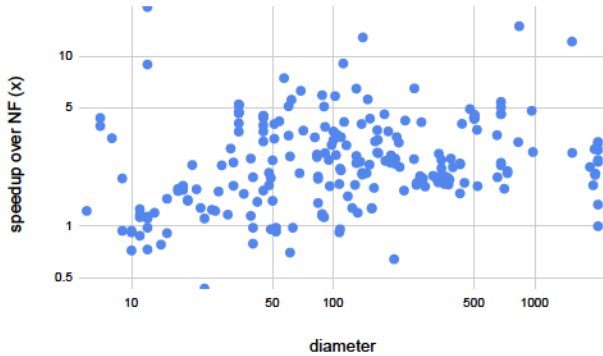
Figure 9. Speedup of ADDS over NF vs. graph diameter.
