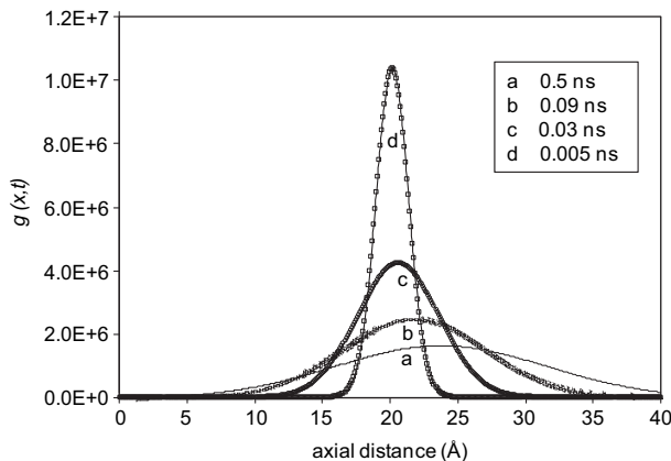
Fig. 3. The figure shows the time diffusion and electric field-influenced variation of the Green function from Eq. (8b). The channel was assumed to be 40 Å long and the initial pulse is applied in the middle of the channel. The pulse decays with time as a result of diffusion and also propagates to the right due to the applied electric field.
