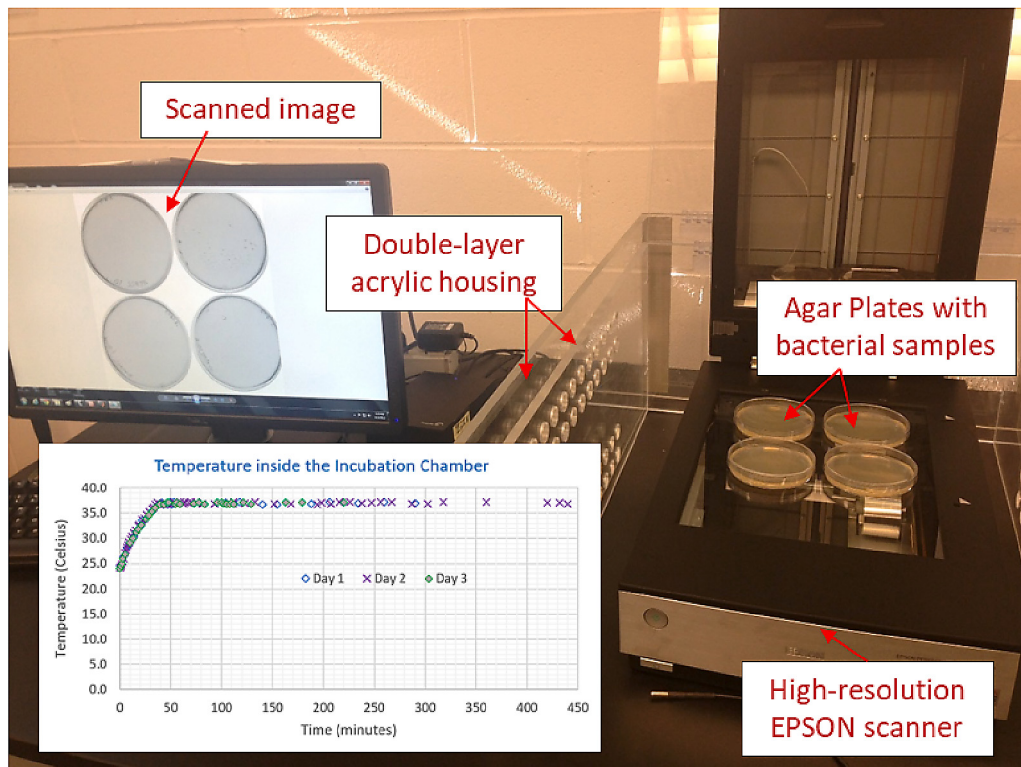
Fig. 1. Open-source hardware to track the growth and imaging of bacterial colonies on agar plates. (A) The enclosure for housing the scanner is shown, along with the heating unit, thermostat to monitor the internal temperature, ventilation tubing, and desktop computer. (B) Four nutrient agar plates are placed on the EPSON flatbed scanner. Scanned image of the four agar plates are displayed on the monitor. The inset shows the temperature within the enclosure as a function of time.
