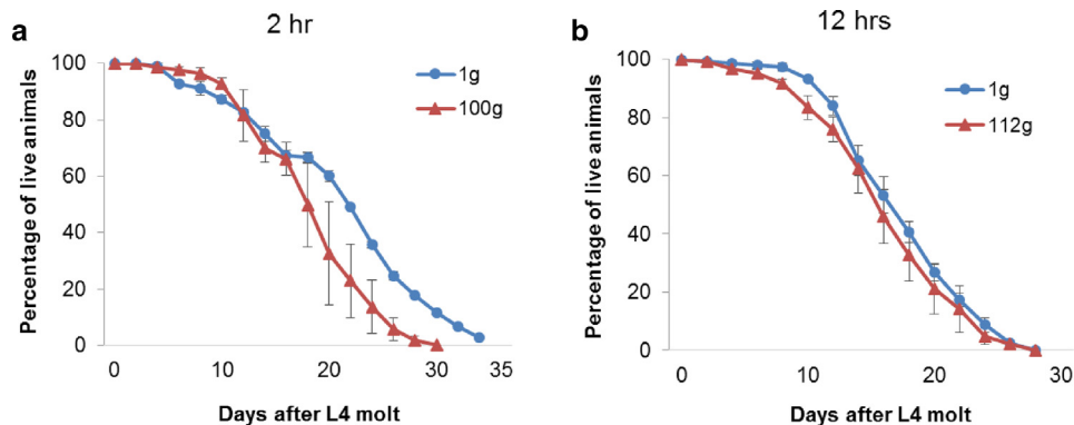
Fig. 5. Effects of 100 g exposure on C. elegans lifespan. The viability of C. elegans was assessed following 100 g hypergravity treatment for 2 h (a) or 112 g hypergravity treatment 12 h (b). Each graph illustrates the survival probability after exposure to hypergravity (red triangles) or control conditions (blue circles). The 100 g hypergravity treatment for 2 h reduced the mean lifespan of the animals ( p < 0.0001 , Log-rank test was used to test for equality of survival distribution). The lifespans of the animals exposed to 12 h of 112 g and 12 h of 1 g controls were similar ( p = 0.1277 , Log-rank test). Further details are provided in Supplementary Table S3. Three independent trials were performed per treatment, and 45–60 animals were tested per trial. Error bars indicate standard error.
