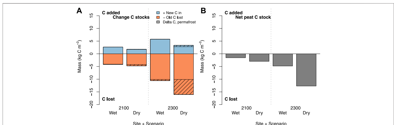
FIGURE 6 | Simplified peat profile diagrams for changes in C stock for the two landscape scenarios (Wet, Dry) in 2100 CE and 2300 CE relative to 2015 CE. (A) Changes in C stocks, including new peat C added (blue) and old peat C lost (orange). The amount of new peat added or old peat lost from permafrost is indicated by the black diagonal stripes. New C additions and old carbon losses are defined as peat deposited before 2015 (old) or after 2015 (new). (B) Net change in peat C stocks in the two landscape scenarios for the two time periods. All scenarios showed a net peat C loss.
