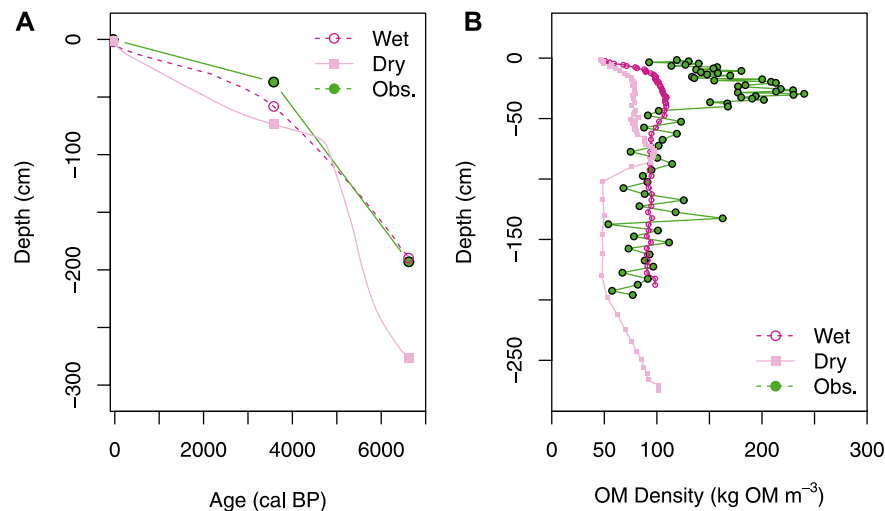
FIGURE 2 | Depth profiles for TKP for modeled scenarios (wet, dry landscapes) and observations (Obs.). (A) Modeled age-depth profiles (light pink and dark pink) are continuous with circles corresponding to the ages of the observations, while the green line connecting the observations is a linear interpolation between the three observed points. (B) Modeled and observed organic matter density with depth.
