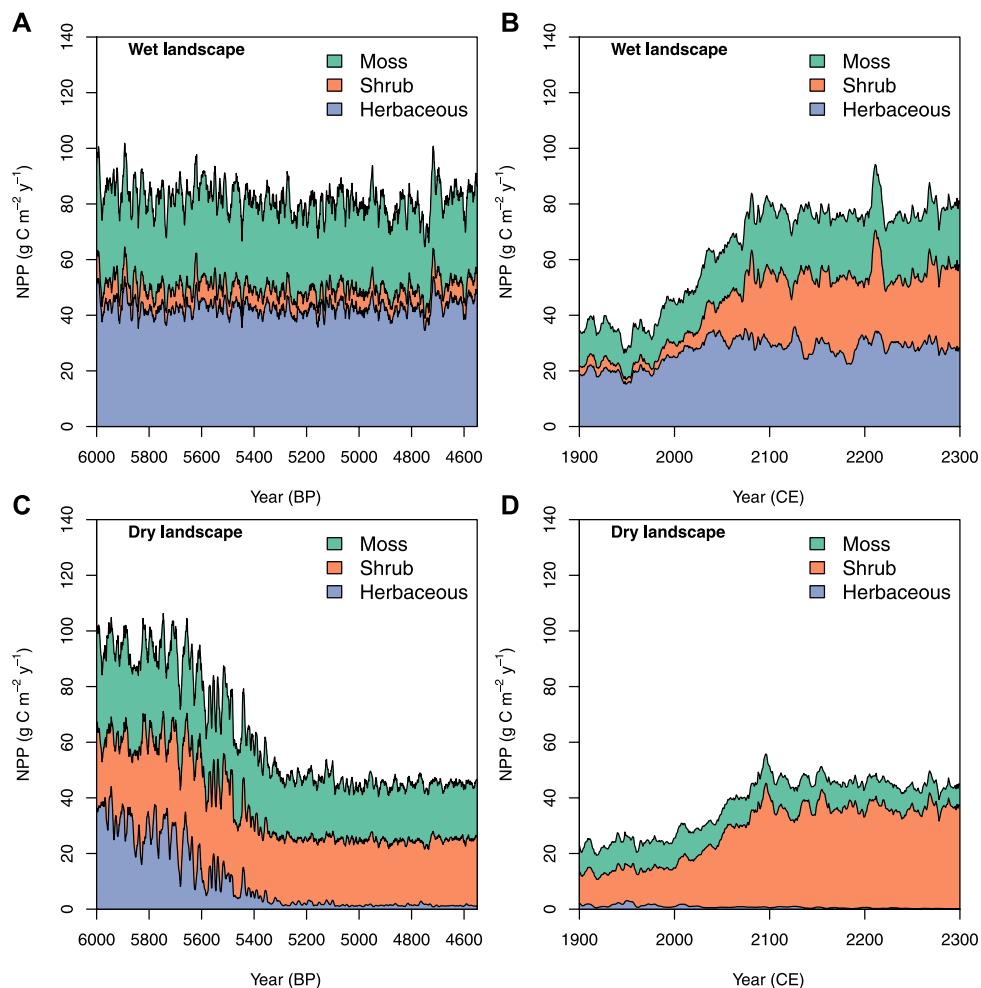
FIGURE 4 | Modeled net primary productivity for moss, shrub, and herb plant functional types in the wet (top) and dry (bottom) landscape scenarios for two time periods: 6,000 BP–4,550 BP (left) and between 1900 and 2300 CE (right). (A) Wet landscape scenario, 6000 - 4550 BP; (B) Wet landscape scenario, 1900 - 2300 CE; (C) Dry landscape scenario, 6000 - 4550 BP; (D) Dry landscape scenario, 1900 - 2300 CE.
