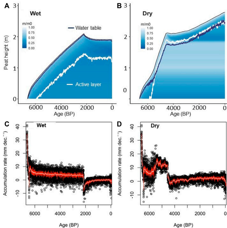
FIGURE 1 | Time series of peat profiles at TKP with two different values of model parameter for the peat height when run-on switches to run-off ( H_{run-on/off} ): (A) H_{run-on/off} = 4.5 results in a wetter peat profile with a water table (blue line) near the peat surface; (B) H_{run-on/off} = 0.5 results in a drier peat profile and an unsaturated (dry) active layer (white line); m/m_0 represents the peat litter cohort mass remaining, high values indicating relatively undecomposed peat; (C) Modeled peat accumulation rates for the wet landscape scenario (black circles), as well as smoothed rates using decadal (red) and centennial (gray) filters; (D) Modeled peat accumulation rates for the dry landscape scenario (black circles), as well as smoothed rates using decadal (red) and centennial (gray) smoothing. All other parameters and climate drivers were the same between the two simulations.
