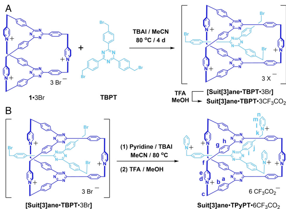
Fig. 5. Mechanistic study. (A) Generation of the reactive intermediate [\text{Suit}[3]\text{ane}\cdot\text{TBPT}\cdot 3\text{Br}]^{3+} and subsequent counterion exchange to give \text{Suit}[3]\text{ane}\cdot\text{TBPT}\cdot 3\text{CF}_3\text{CO}_2^- . This compound, however, can be easily hydrolyzed at room temperature so only mass spectrum was recorded. (B) Capturing of the reactive intermediate [\text{Suit}[3]\text{ane}\cdot\text{TBPT}\cdot 3\text{Br}]^{3+} by reacting it with pyridine in the presence of TBAI to form \text{Suit}[3]\text{ane}\cdot\text{TPyPT}\cdot 6\text{CF}_3\text{CO}_2^- , which is stable during column purification using \text{H}_2\text{O} and MeCN as the eluent and can be fully characterized.
