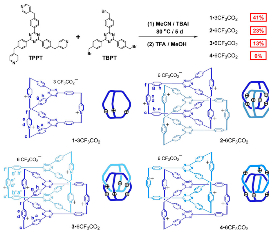
Fig. 2. One-pot syntheses of the monomeric cage 1\cdot 3\text{CF}_3\text{CO}_2 and the 3D catenanes 2\cdot 6\text{CF}_3\text{CO}_2 and 3\cdot 6\text{CF}_3\text{CO}_2 from TPPT and TBPT using TBAI as a catalyst. The formation of another putative 3D catenane 4\cdot 6\text{CF}_3\text{CO}_2 was, however, not observed.
