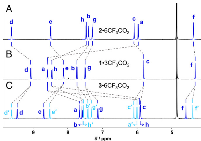
Fig. 3. Structural elucidation of 1\cdot3\text{CF}_3\text{CO}_2 , 2\cdot6\text{CF}_3\text{CO}_2 and 3\cdot6\text{CF}_3\text{CO}_2 by ^1\text{H} NMR (500 MHz, 298 K, \text{CD}_3\text{OD} ) spectroscopy. ^1\text{H} NMR spectra of (A) 2\cdot6\text{CF}_3\text{CO}_2 , (B) 1\cdot3\text{CF}_3\text{CO}_2 , and (C) 3\cdot6\text{CF}_3\text{CO}_2 . The resonances corresponding to \text{H}_a (5.97 ppm) in 2\cdot6\text{CF}_3\text{CO}_2 , and \text{H}_{a'} (6.01 ppm) and \text{H}_h (5.91 ppm) in 3\cdot6\text{CF}_3\text{CO}_2 show significant upfield shifts compared with those (8.58 ppm for \text{H}_a and 8.46 ppm for \text{H}_h ) in 1\cdot3\text{CF}_3\text{CO}_2 . This observation is good evidence for the formation of MIMs, in which the inside protons are shielded by the other cage component.
