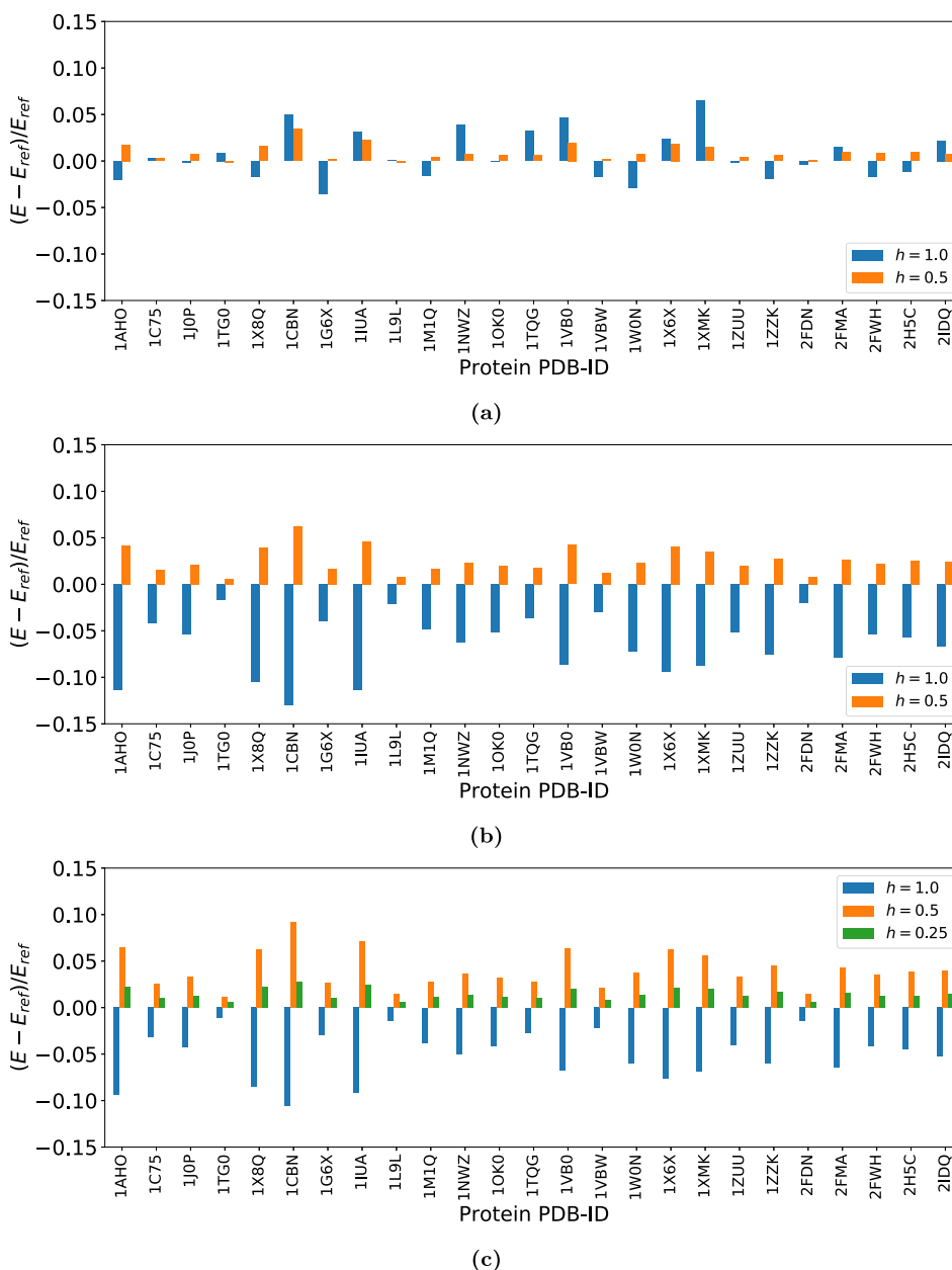
Fig. 8. (a) Self-convergence of the regularization energy. Here E_{ref} is the regularization energy at h = 0.25 , and E is the regularization energy at h = 1 or 0.5 ; (b) Self-convergence of the trilinear energy. Here E_{ref} is the trilinear energy at h = 0.25 , and E is the trilinear energy at h = 1 or 0.5 ; (c) Convergence of the trilinear energy toward the regularization energy. Here E_{ref} is the regularization energy at h = 0.25 , and E is the trilinear energy at h = 1 , 0.5 , or 0.25 .
