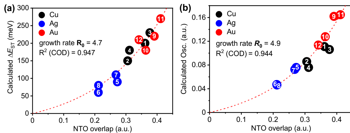
Figure 5. Relationship between ^1\text{ICT} NTO overlap value versus theoretically calculated (a) \Delta E_{ST} and (b) oscillator strength of the S_1 state by TD-DFT method; fits to the data are obtained using the exponential growth function: y = A(e^{R_0x} - 1) .
