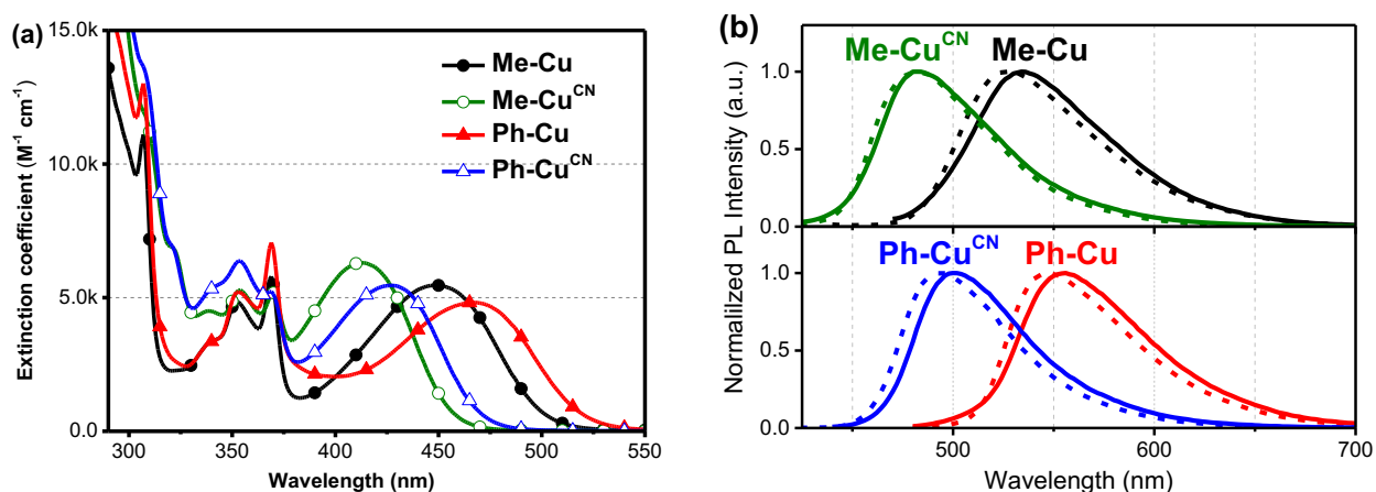
Figure 3. (a) Absorption and (b) emission spectra of Cu-based complexes. Absorption spectra recorded in toluene solution at room temperature and emission spectra in doped PS (1 wt%) films at room temperature (solid) and 77 K (dash).
