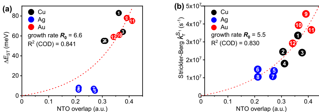
Figure 6. Relationship between ^1\text{ICT} NTO overlap value versus (a) \Delta E_{\text{ST}} and (b) radiative decay rate of the ^1\text{ICT} state according to the Strickler-Berg equation; fits to the data are obtained from on the twelve complexes in this work using the exponential growth function: y = A(e^{R_0x} - 1) .
