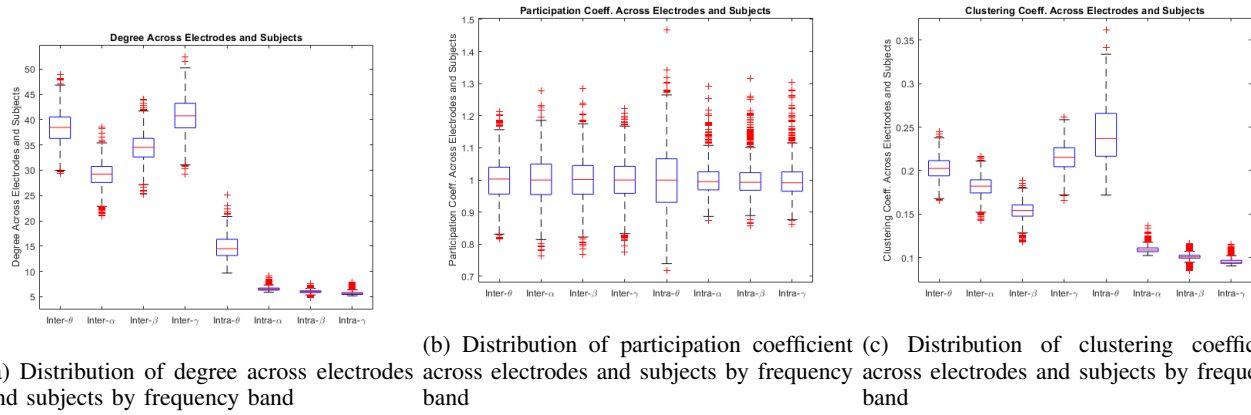
Fig. 1: Box plots representing three different metrics: degree, participation, clustering coefficient, averaged across electrodes and subjects by frequency band.
