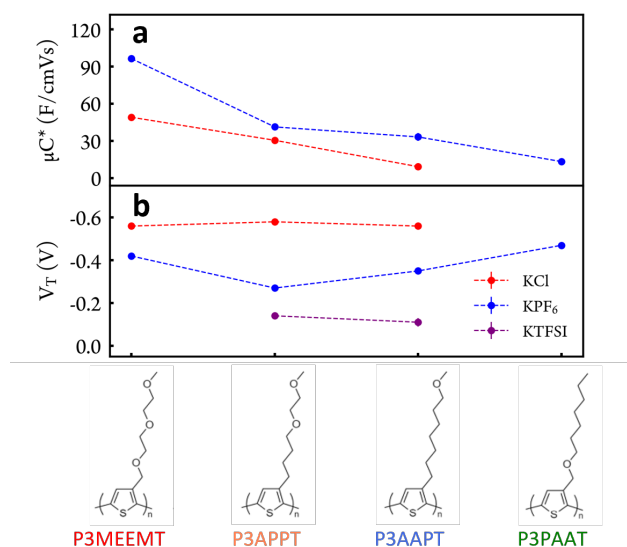
Figure 2. (a) OECT material figure of merit \mu C^* and (b) OECT threshold voltage ( V_T ) in 100 mmol/L KCl(aq) (red), KPF 6 (aq) (blue) and KTFSI (purple). Dash lines are guide for the eye.
