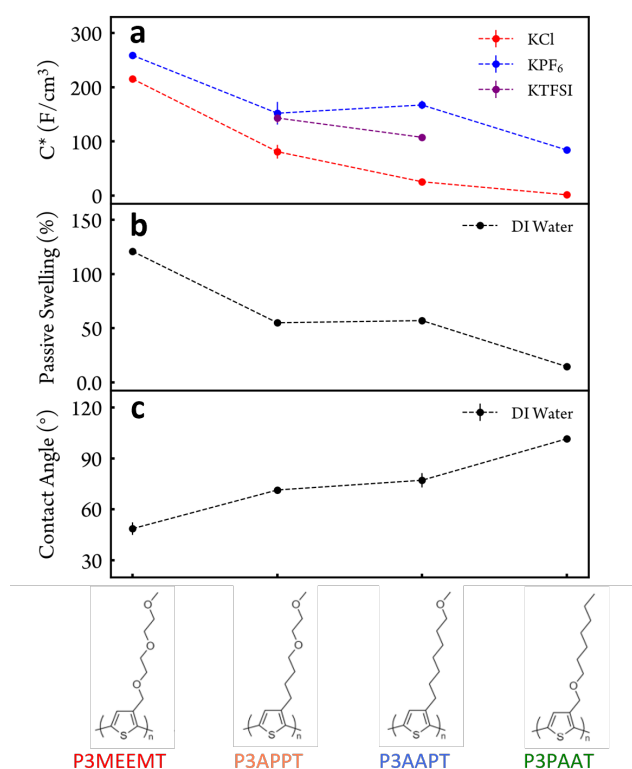
Figure 4. (a) Volumetric capacitance C^* in 100 mmol/L \text{KCl}_{(\text{aq})} (red), \text{KPF}_{6(\text{aq})} (blue) and \text{KTFSI} (purple). (b) Passive swelling of polymers in DI water. We did not observe significant difference of passive swelling in \text{KCl}_{(\text{aq})} , \text{KPF}_{6(\text{aq})} or DI water. (c) Water contact angle of polymers. Dash lines are guide for the eye.
