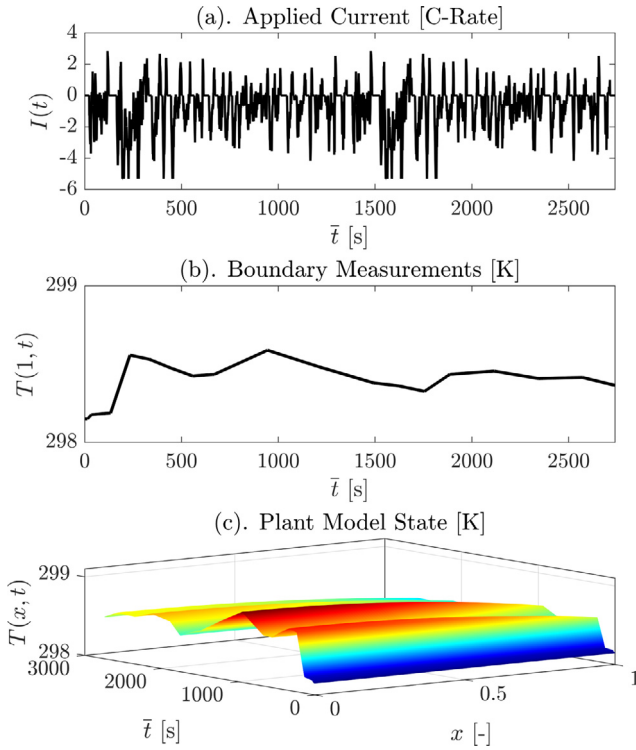
Fig. 4. The plant model response under a FUDS drive cycle. Plant model initial condition: T_0(x) = T_{\text{amb}} = 298.15 K for all x \in [0, 1] .
