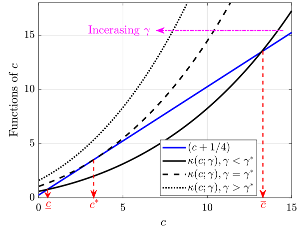
Fig. 1. An illustration of design parameter selection to guarantee observer convergence. As \gamma increases, the function \kappa(c; \gamma) shifts towards the upper-left direction and the span between c = \underline{c} and c = \bar{c} shrinks accordingly. When \gamma < \gamma^* \approx 1.053 , it is ensured that there always exists a design parameter c such that the conditions in (57) hold. (For interpretation of the references to color in this figure legend, the reader is referred to the web version of this article.)
