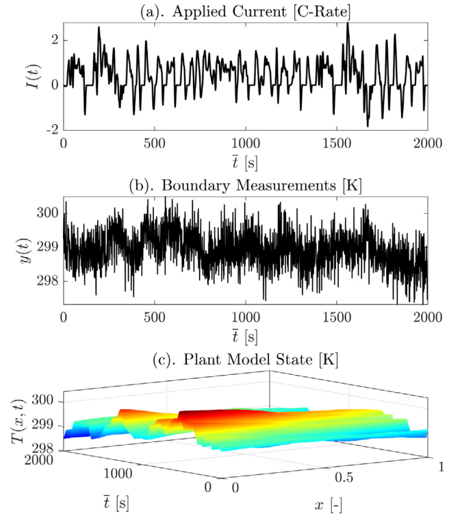
Fig. 6. The plant model response under a UDDS drive cycle. Plant model initial condition: T_0(x) = T_{\text{amb}} + 1 K = 299.15 K for all x \in [0, 1] . Gaussian noise with 0.3 K variance and zero mean, i.e., \mu(t) \sim \mathcal{N}(0, 1) , is injected to the boundary measurement signal y(t) . Uniformly distributed random noise \varepsilon(x, t) is introduced into the plant model (14).
