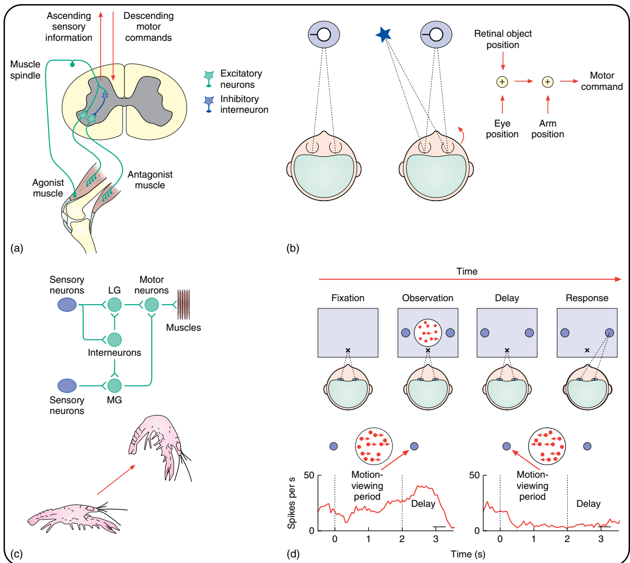
Figure 4 (a) The knee-jerk reflex relies on direct synaptic connections between sensory and motor neurons. Muscle spindles that sense the stretch of the quadriceps muscle resulting from tapping the knee tendon excite a pool of motor neurons in the spinal cord causing contraction of the quadriceps (agonist) and inhibit a pool of motor neurons that contract the antagonist muscle via interneurons. This information is conveyed to the brain by ascending pathways. More complex voluntary behaviours such as reaching are controlled by descending pathways conveying motor commands from the brain. (b) Coordinate transformations are essential for proper execution of motor programmes. If a subject fixes a cup directly (left panel), its position on the retina will be different than if the subject is looking at something else (right panel). The retinal position of the cup must therefore be combined with eye position information relative to the head to provide the appropriate motor command moving the arm. (c) The crayfish tail-flip escape response illustrated at the bottom is mediated by a simple circuit comprising a pair of neurons on each side of the body called the lateral giant fibre (LG) and the medial giant fibre (MG). A single action potential in any of these neurons causes the activation of motor neurons in several body segments, resulting in the escape behaviour. Sensory neurons innervating LG and MG originate in part from different body segments. Interneurons play an important role in shaping the timing of the response. Adapted from Edwards et al. (1999), with permission from Elsevier Science. (d) Response of a neuron in a premotor cortical area during a direction discrimination task. The monkey observes a motion signal consisting of dots moving in either of two directions and is trained to report the direction of motion by an eye movement after a delay. The particular neuron illustrated at the bottom shows strong activity during the delay period for an eye movement to the right but not for an eye movement to the left, thus revealing the intention of the monkey. Adapted from Leon and Shadlen (1998) Neuron 21: 669–672, with permission from Cell Press.
