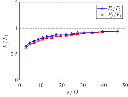
FIG. 4. Force acting on the leading rod F_l and the following rod F_f normalized by the force acting on a single rod F_1 in a viscous Newtonian fluid. F_l tends to be slightly higher than F_f at lower s/D but are overall nearly indistinguishable from one another ( Re = 2.5 \times 10^{-1} ).
