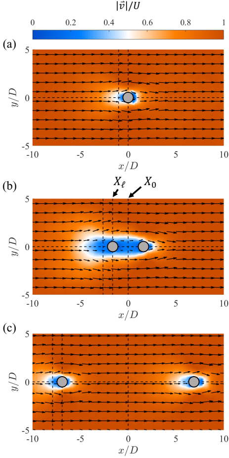
FIG. 6. Mean flow field normalized by the imposed velocity of U = 1.3 \text{ mm/s} or about 0.4D/s at depth z_o = 5d . Flow is moving from left to right, as indicated by the velocity vectors. (a) Flow past one rod shows a left-right-asymmetry, where particles slow down in a conical shape in front of the rod. (b) Flow past two rods with s/D = 5.5 . A strong interaction between the two rods is noted by the region between the rods that is 50% slower than the imposed velocity. (c) Flow past two rods with s/D = 11 . The flow field around the two rods are independent from each other. The two vertical dotted lines X_0 and X_1 are denoted as the line equidistant from the two rods and the line that passes through the leading rod, respectively. The horizontal dotted line passes through the two rods along y/D = 0 . Velocity profiles along these lines are shown in Fig. 7 and 8.
