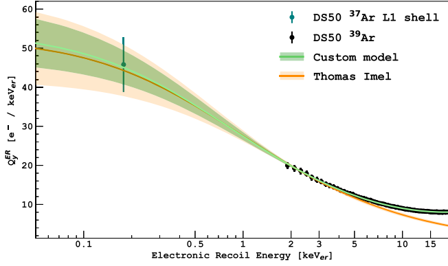
FIG. 2. Fit of the ER ionization yield, measured from AAr (black) and ^{37}\text{Ar} (teal) data with a drift field of 200 V/cm, with the Thomas-Imel box model up to 3 keV er [Eq. (4)], and with the custom model from Eq. (6), which extends the Thomas-Imel model up to 20 keV er . The model bands correspond to 1\sigma , also accounting for the correlation from the g_2 systematics, which dominates the experimental uncertainties.
