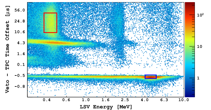
FIG. 6. Veto selection of prompt (blue box) and delayed (red box) events associated to AmBe neutron emission, as a function of liquid scintillator veto (LSV) visible energy and time difference between veto and TPC signals. The trigger time offset between the two detectors is about -550 ns. The horizontal feature at the 4.3 \mu\text{s} offset is due to PMT afterpulses.
