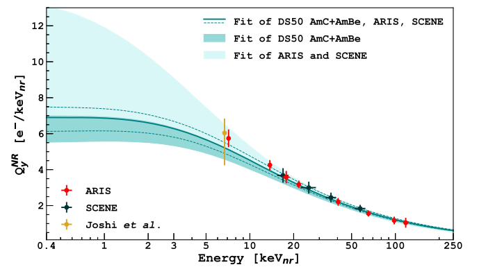
FIG. 8. Fit of the NR ionization yield at 200 V/cm from the combined fit of DarkSide-50 AmBe and AmC calibration data, together with datasets from SCENE [39] and ARIS measurements [35], the latter combined with the DarkSide-50 ionization-to-scintillation ratio. The measured Q_y^{\text{NR}} by Joshi et al. [40] at 6.7 keV nr is reported for comparison. The model bands correspond to 1\sigma uncertainty.
