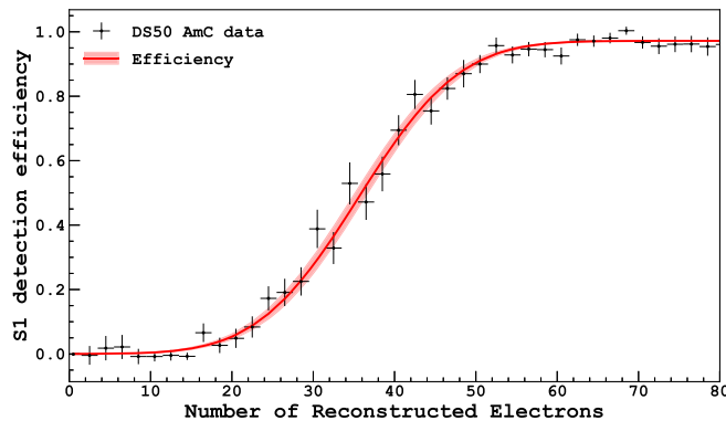
FIG. 5. Efficiency in detecting S1 + S2 events ( N_{2p} ) with respect to S1 + S2 and S2 only ( N_{1p} ), as a function of the reconstructed number of electrons. Data are fitted with an error function (red line). The error band is propagated from the uncertainties of the fitted parameters.
