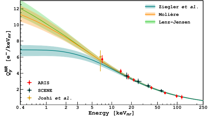
FIG. 10. Fit of DarkSide-50 AmBe and AmC data, and ARIS and SCENE datasets using Ziegler et al. [Eq. (13)] [37], Molière [43], and Lenz-Jensen [44,45] screening functions. The model bands correspond to 1\sigma uncertainty.
