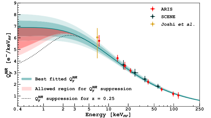
FIG. 11. Allowed region (red) for low energy Q_y^{\text{NR}} suppression tested on the AmC dataset, and best-fitted Q_y^{\text{NR}} (blue), using the Ziegler et al. screening function. Dark (light) shaded area corresponds to 1\sigma ( 2\sigma ) uncertainty. The dashed line represents the Q_y^{\text{NR}} suppression tested in [36] assuming Eq. (16) with z = 0.25 .
