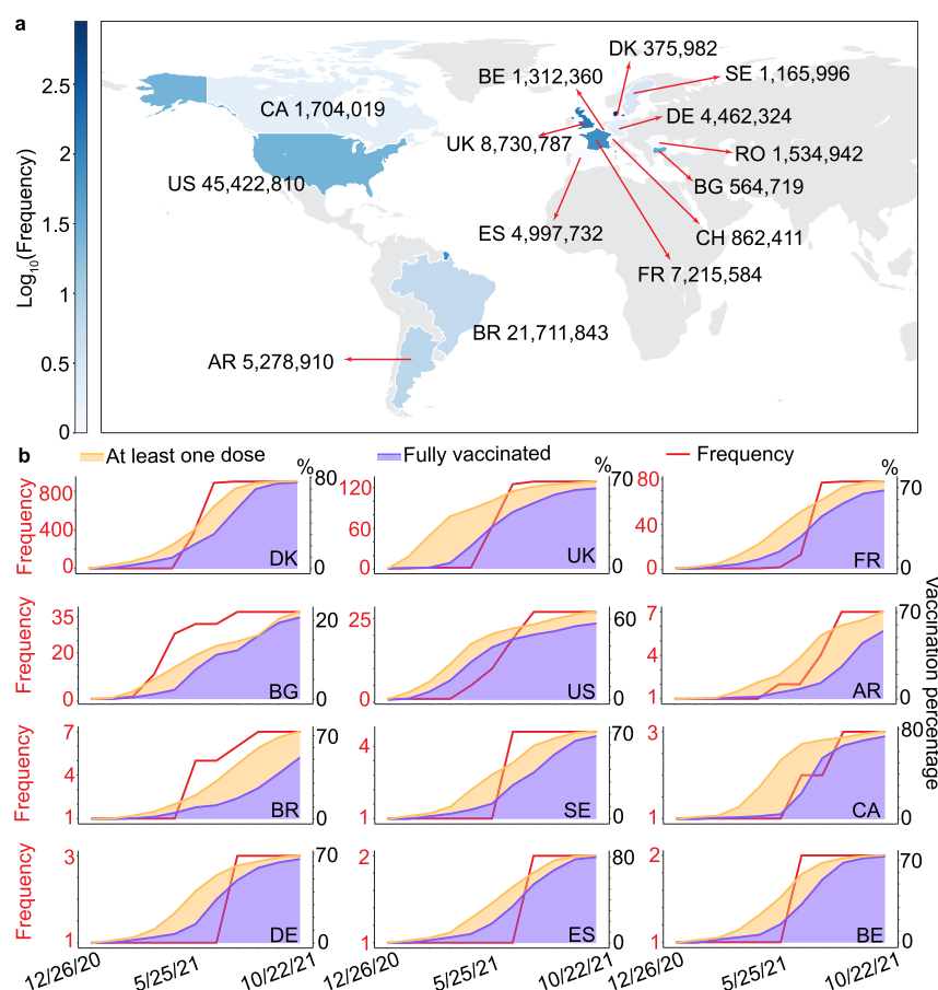
Figure 4. (a) Distribution of vaccine-resistant mutation Y449S. The color bar represents the \log_{10} frequency of Y449S in 14 countries: Denmark (DK), the United Kingdom (UK), France (FR), Bulgaria (BG), the United States (US), Argentina (AR), Brazil (BR), Sweden (SE), Canada (CA), Switzerland (CH), Germany (DE), Spain (ES), Romania (RO), and Belgium (BE). The number located at the side of the country shows the total number of positive SARS-CoV-2 cases by October 22. (b) Time evolution of the vaccination rate and the frequency of Y449S in top 12 countries from December 26, 2020, to October 22, 2021. The data are collected per 30 days. The red line shows the frequency of mutation Y449S. The orange and purple areas represent the rate of at least one dose and the rate of full vaccination, respectively, in each country.
