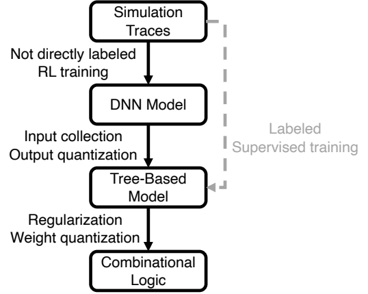
Fig. 1: Proposed flow of distilling logic from traces. For supervised tasks, tree models can be directly trained from simulation traces. This paper focuses on converting deep learning models to circuits.
