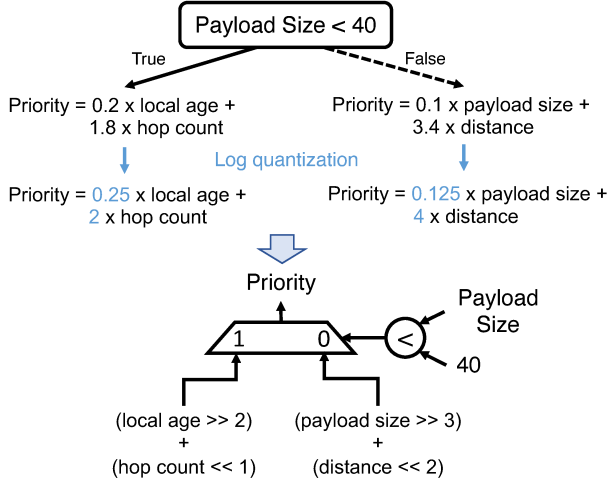
(b) Convert linear model tree to logic.
