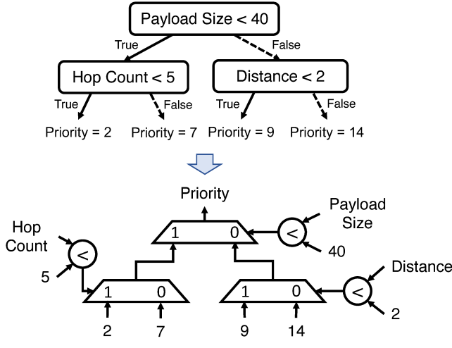
(a) Convert decision tree to logic.
