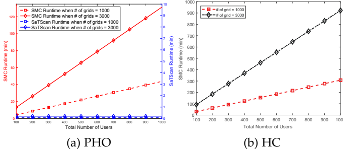
Figure 6: Computation overhead for PHO and HC.
