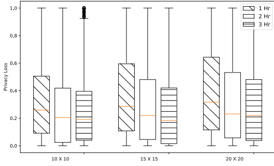
Figure 5: Privacy loss per-user under different inference settings.
