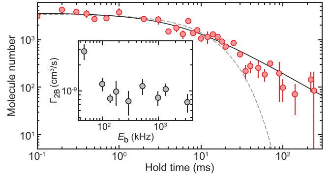
FIG. 5. Lifetime of NaCs Feshbach molecules. Decay dynamics are recorded for molecules at a binding energy of h \times 1.3 MHz. The solid (dashed) line is a fit to two-body (one-body) decay. The inset shows the derived two-body loss coefficients as a function of molecular binding energy for a cloud temperature of 1.8(4) \mu\text{K} . We attribute the increased decay at E_b = h \times 50 kHz to thermal dissociation of Feshbach molecules as the binding energy is comparable to the temperature.
