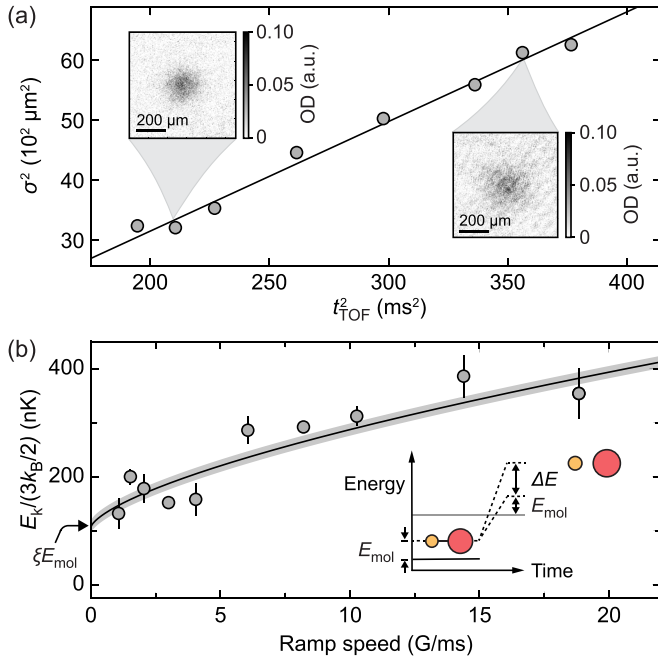
FIG. 3. Measuring the mean kinetic energy of NaCs Feshbach molecules. (a) Cloud size \sigma vs time of flight t_{TOF} for a dissociation ramp speed of 10 G/ms. \sigma is obtained from a two-dimensional Gaussian fit to the Cs clouds after dissociation. The solid line shows a linear fit where the slope equals to \Delta\sigma^2/\Delta t_{TOF}^2 (see text). (b) Mean kinetic energy of the resulting Cs cloud vs ramp speed. The solid line shows a fit of \xi E_{mol} + \Delta E(\dot{B}) , where E_{mol} is the only fitting parameter. For this data set, the fit yields T_{mol} = 124(13) nK.
