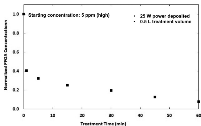
FIG. 14. Forever chemical PFOA removal via batch processing with packed bed reactor. 43
