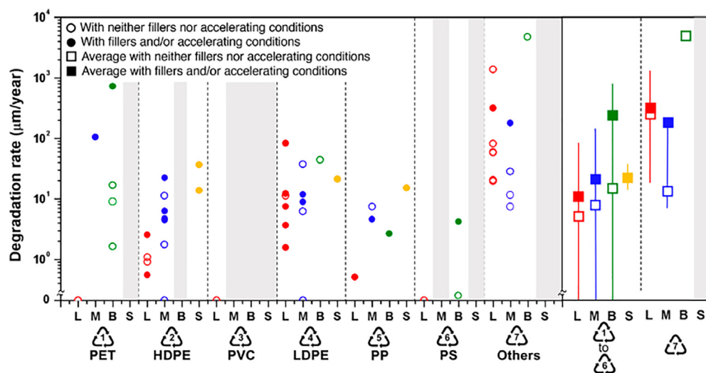
FIG. 16. Degradation rates for different types of plastics, where letters designate degradation environment. L: landfill, M: marine, B: biological degradation, and S: sunlight. 53
