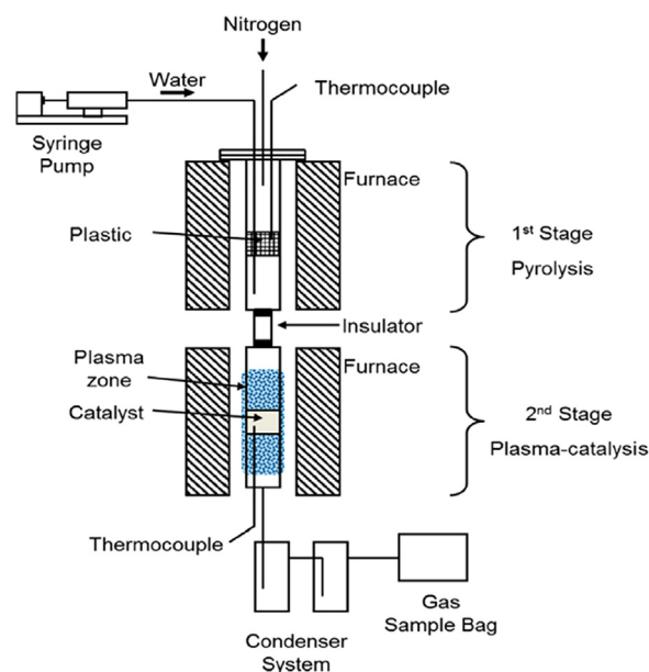
FIG. 18. Dual-stage thermal pyrolysis nonthermal plasma reactor for polymer treatment. 70
