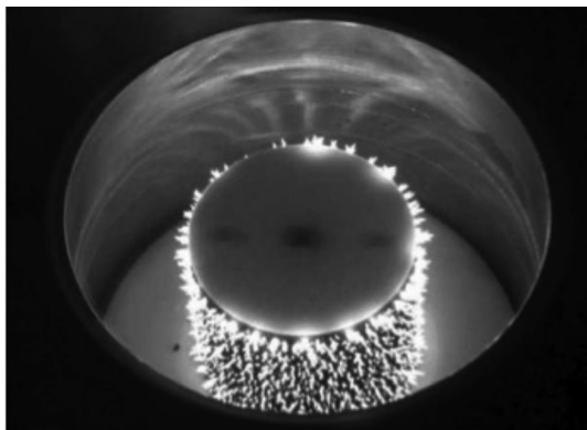
FIG. 4. Pulsed corona discharge geometry and operation. 8 [Adapted with permission from Lukes et al. , Plasma Processes Polym. 6 , 719 (2009). Copyright 2009 Wiley.]
