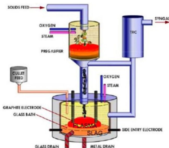
FIG. 17. Plasma pyrolysis reactor for gasification of plastics. 61
