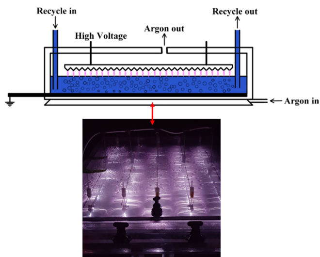
FIG. 11. Multi-appligator argon gas discharge for the treatment of PFAS in water. 41
