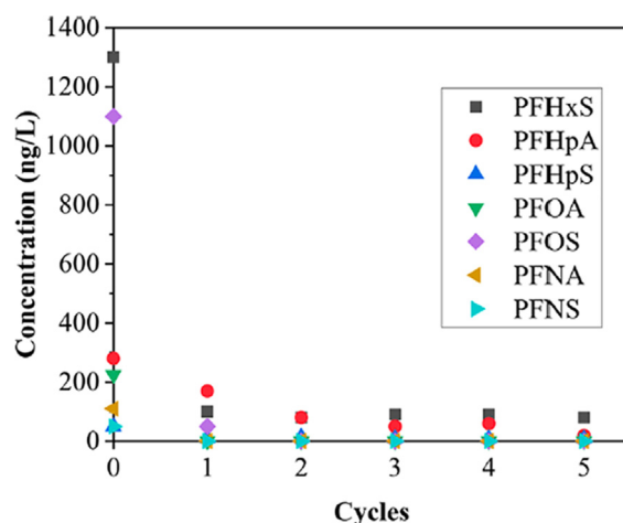
FIG. 12. Decomposition of a range of PFAS contaminants as a function of cycles through the reactor. 41
