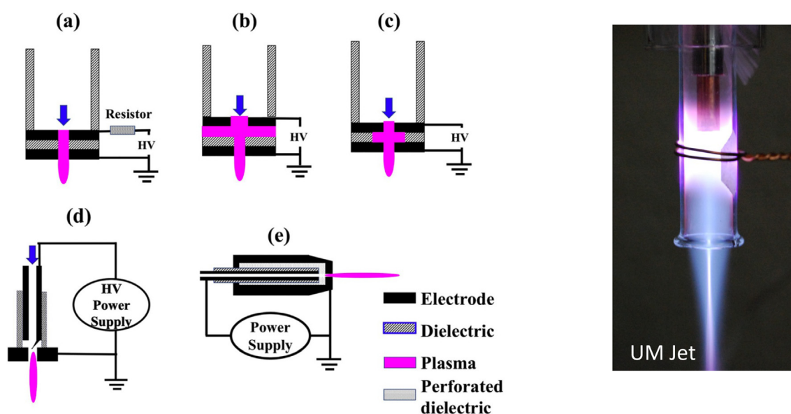
FIG. 5. Plasma jet implementations 11 [Adapted with permission from Lu et al. , Phys. Plasmas 28 , 100501 (2021). Copyright 2021 AIP Publishing LL] and photograph of operating jet from PSTL UM lab-B. Yee.
