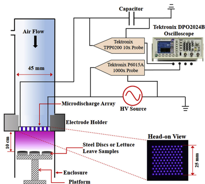
FIG. 24. Air plasma generated by a two-dimensional array of integrated coaxial-microhollow dielectric barrier discharge, designed for food decontamination. 121
