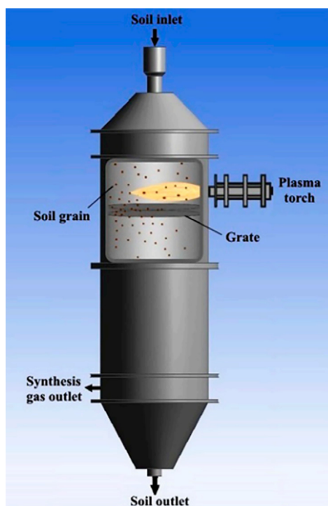
FIG. 28. Plasma reactor for soil decontamination. 166
