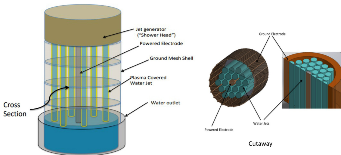
FIG. 13. Cutaway of packed bed plasma water reactor. Plasma flows along water streams as surface ionization waves. 43
