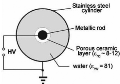
FIG. 4. Pulsed corona discharge geometry and operation. 8 [Adapted with permission from Lukes et al. , Plasma Processes Polym. 6 , 719 (2009). Copyright 2009 Wiley.]
