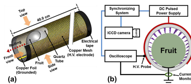
FIG. 23. Atmospheric pressure air dielectric barrier discharge for decontamination of rolling fruits. 96
