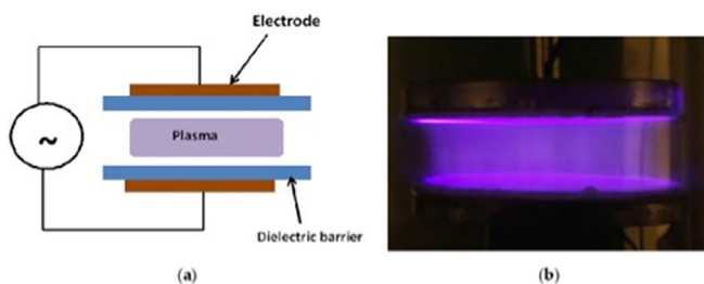
FIG. 3. Schematic depiction of dielectric barrier discharge along with photograph of operating discharge.
