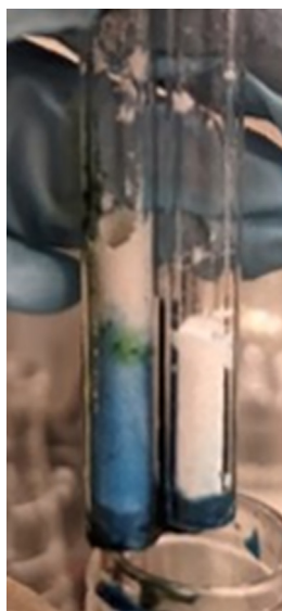
FIG. 21. In-house PET powder exposed to blue dye for Washburn capillary rise test, showing greatest rise in plasma treated sample on left suggesting increased hydrophilicity. 77 (R. Pinsky).
