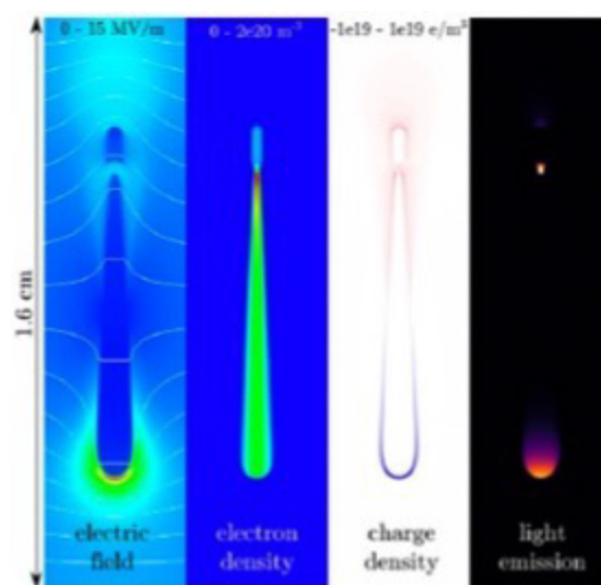
FIG. 2. Simulation of a positive streamer propagating downward (exciting voltage 32 kV in 1 atm). 5
