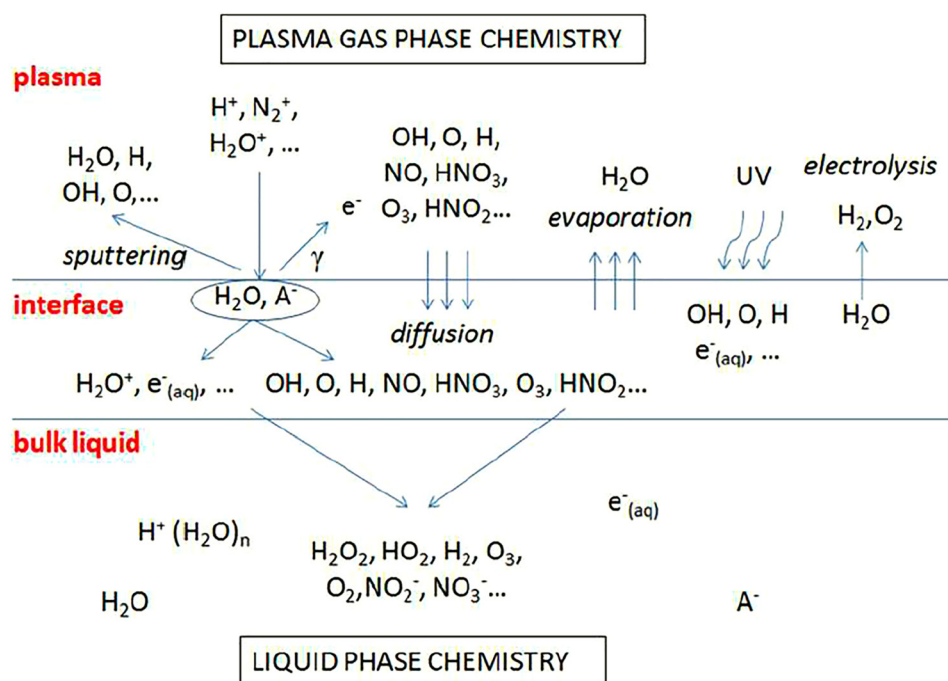
FIG. 10. Complex processes occurring at interface of plasma with liquid water. 39
