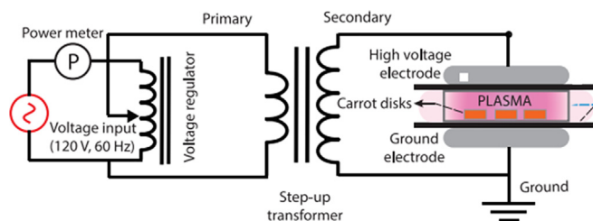
FIG. 25. Experimental setup for in-package DBD plasma treatment of carrot disks. 137
