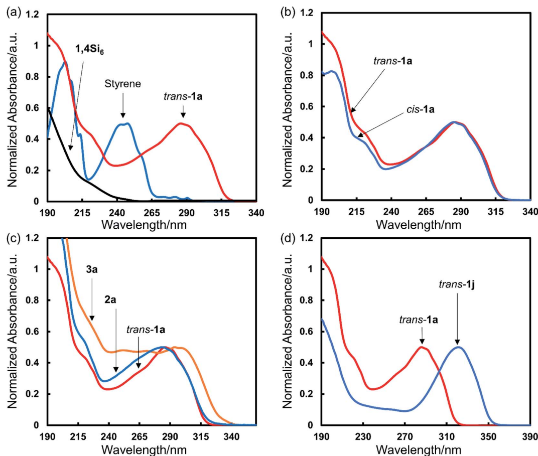
Fig. 6 UV-vis spectra with normalized absorbance ([compound] = 10^{-5} \text{ M} , in n -pentane). (a) Comparison to starting material. Red: trans - 1a ; black: 1,4Si 6 ; blue: styrene. (b) Influence of configuration. Red: trans - 1a ; blue: cis - 1a (dr 25 : 75 trans : cis ). (c) Cyclosilane comparison. Red: trans - 1a ; blue: 2a (dr 55 : 45 trans : cis ); orange: 3a . (d) Heterocycle effect. Red: trans - 1a ; blue: 1j (dr 90 : 10 trans : cis ).
