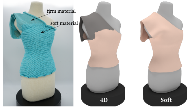
Fig. 17. One-shoulder knitted top with prescribed material distribution to achieve a desired shape. Firm material on the shoulder produces a stiff style, while soft material on the torso ensures comfort. From the simulation, it can be found that the style cannot be achieved using a uniformly soft material.
