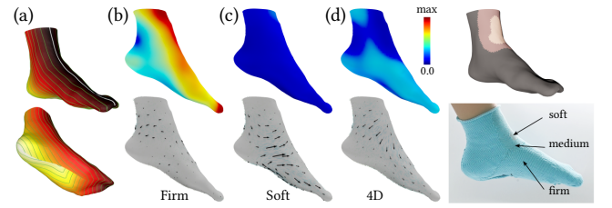
Fig. 16. Sock with distributed elasticity: (a) geodesic distance-field for generating the stitch mesh, (b) simulation of 3D knitting with firm material, (c) simulation of 3D knitting with soft material, (d) resulting 4D design with simulation and physical experiments. Both the stresses and the displacements have been significantly reduced. The maximal stress in this example is 0.6602kPa. The try-on process of this 4D sock can be found in the supplementary video. In this example, \bar{d} = 0.8\text{cm} is employed as the terminal threshold of inverse design.
