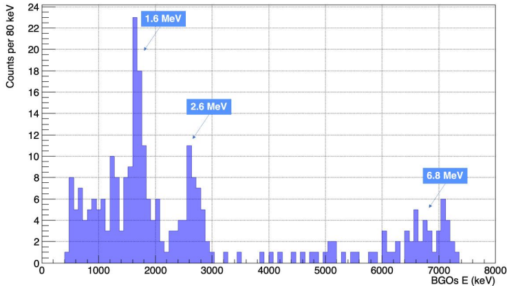
Figure 4. BGO spectrum gated on the events of the BGO - Si time difference peak corresponding to the recoil ToF. The \gamma -rays of the ^{20}\text{Ne} 11.09 MeV level decay cascade can be clearly seen at 1.633, 2.613, and 6.841 MeV.
