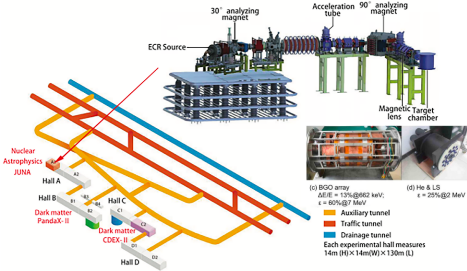
Figure 1. The layout of JUNA in CJPL-II
