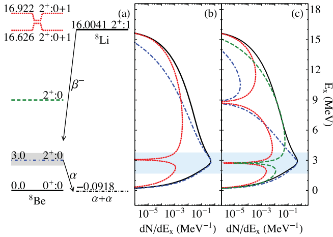
FIG. 1. (a) The \beta -decay scheme of ^8\text{Li} (with E_x , J^\pi , and T listed from left to right) [17]. Sample ^8\text{Be} excitation energy E_x spectrum R -matrix fits (black) with approximate individual state contributions from (b) the 3-MeV resonance (blue) and doublet states (red) and (c) with an intruder state (green) centered at \sim 9 MeV added. The region highlighted in blue is the E_x range used in our analysis.
