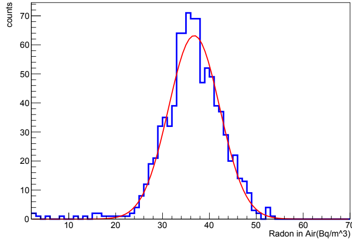
Figure 7. The variation of the radon monitoring over two and a half years of data collection. A Gaussian fit is overlaid on the measurement. The fit mean and standard deviation are 36.7 and 5.5 Bq/m 3 , respectively.
