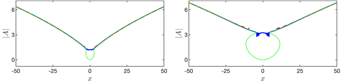
Figure 16: Spatial profiles of |A| (blue curves) for the same solution as in Figure 15 at \mu = 1.5 and \mu = 10.5 . The oscillations are seen in the center of the domain, and the width of this central region increases slowly: -2 \lesssim x \lesssim 2 at \mu = 1.5 and -3 \lesssim x \lesssim 3 at \mu = 10.5 . Outside these central intervals, the solution is close to the repelling QSS, which is given to leading order by (8.2)(b) (dashed red curve). Super-imposed is the numerically obtained solution (green curve) of the leading order QSS equation, r^2 ((\mu - r^2)^2 + (\omega_0 - \alpha r^2)^2) = \varepsilon x^4 , valid for all x , as obtained from (1.1) by neglecting the time and space derivative terms (which are higher order) and then squaring the modulus. Here, r = |A| , \mu is real, and \alpha = 0 . On |x| \gg \varepsilon^{-\frac{1}{4}} , the green curve lies essentially on top of the blue and red curves. For \mu < \omega_0 , the green curve does not have any fold points, and there are no oscillations in the PDE solution, consistent with the DHB analysis. Then, the fold points first appear when \mu reaches \omega_0 to leading order, and they are present (data not shown) for all \mu up until at least 10.5. These fold points delimit the interval on which the oscillations are observed.
