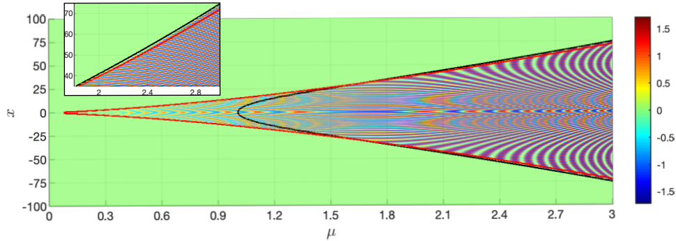
Figure 8: \text{Re}(A) of the solution obtained from the direct numerical simulation of (1.1) with \omega_0 = 1 and source term I_G(x) = e^{-\frac{x^2}{4\sigma}} , \sigma = \frac{1}{4} . The initial data A_0(x) = -\sqrt{\varepsilon} \frac{I_G(x)}{\mu_0 + i\omega_0} is given at \mu_0 = -0.2 . For each x , the solution stays near the repelling QSS (green region) for a long time past the instantaneous Hopf bifurcation at \mu = 0 . Then, the exit time from a neighbourhood of the repelling QSS is x -dependent. In the center, it is given by (4.3) (red curve), where \mu_h(x) < \mu_{\text{stbc}}(x) . In contrast, for x outside this interval, \mu_{\text{stbc}}(x) comes first, and the space-time buffer curve (3.8) (black curve) determines the exit time. The inset shows a magnification for \mu > 1.8 . The convex hull given by (x, \mu = \min(\mu_h(x), \mu_{\text{stbc}}(x))) agrees to leading order with the onset of oscillations for all x . Here, \varepsilon = 0.01, \omega_0 = 1, \alpha = 0.6, d_R = 1, d_I = 0 .
