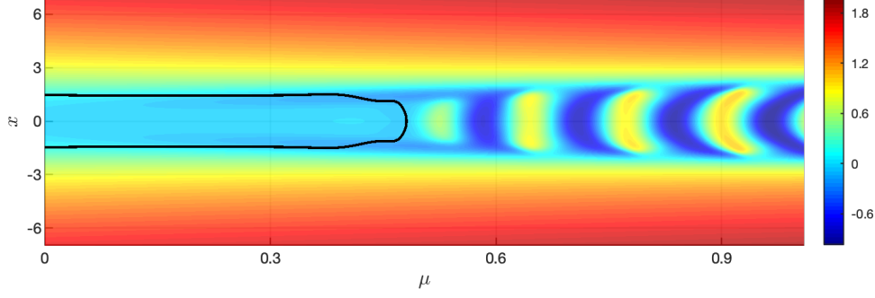
Figure 15: \text{Re}(A(x, \mu)) of the solution of the cubic CGL (1.1) with the algebraically-growing source term, I_{\text{ag}}(x) , along with the exact space-time buffer curve (black curve, given by the exact solution A_p(x, \mu) in (8.5)). DHB and the attendant oscillations are observed in the central portion of the domain ( |x| \lesssim 1.55 ) to the right of the exact space-time buffer curve. These oscillations propagate outward from x = 0 , until they reach |x| \approx 1.5 . For |x| \approx 1.5 , \mu_{\text{stbc}}(x) \approx 0 . Then, outside this central region, the solution stays near the repelling QSS, at least until \mu = 10.5 . Note that the color scale differs from that in the previous figures. The initial data at \mu_0 = -1 is A_0(x) = -\sqrt{\varepsilon} \frac{I_{\text{ag}}(x)}{\mu_0 + i\omega_0} . Here, \omega_0 = \frac{1}{2} , \alpha = 0 , d_R = 1 , and d_I = 0 .
