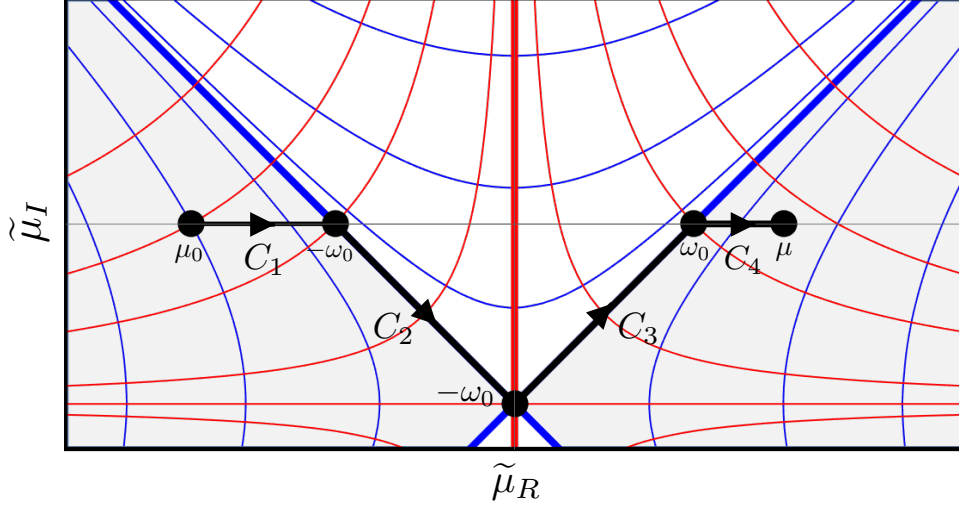
Figure 4: The contour C = C_1 \cup C_2 \cup C_3 \cup C_4 in the complex \tilde{\mu} plane.
