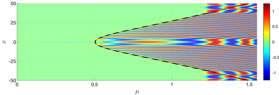
Figure 9: Illustration of DHB in Case 2 showing \text{Re}(A(x, \mu)) obtained from (1.1) with I_G(x) . The initial data is given at time \mu_0 = -1.2 . For |x| \lesssim 37.1 , \mu_{\text{stbc}}(x) < -\mu_0 = +1.2 . Hence, the space-time buffer curve given by the particular solution determines the exit time to leading order for these points x . In contrast, for |x| \gtrsim 37.1 , \mu_{\text{stbc}}(x) > -\mu_0 = +1.2 , so that for these x the exit time is determined to leading order by A_h(x, \mu) . Here, \varepsilon = 0.01, \omega_0 = \frac{1}{2}, d_R = 3, d_I = 1, \alpha = 0.6 , and A_0(x) = \cos\left(\frac{10\pi x}{\ell}\right) with \ell = 50 . Similar results are obtained for other initial data.
