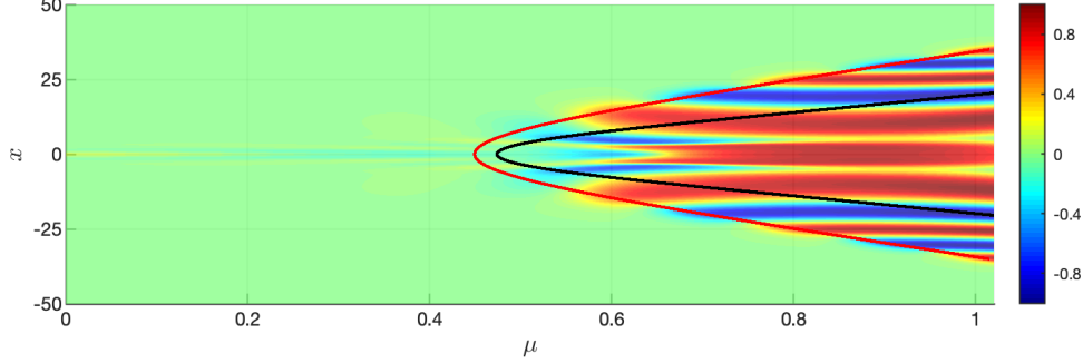
Figure 11: \text{Re}(A(x, \mu)) illustrating DHB in Case 3 for (1.1) with I_G(x) ( \sigma = \frac{1}{4} ). The curves \mu_h(x) (red) and \mu_{\text{stbc}}(x) (black) are super-imposed. For all x in [-\ell, \ell] ( \ell = 50 ), \mu_h(x) < \mu_{\text{stbc}}(x) . Hence, A_h is the first to stop being exponentially small and grow, before A_p does, for each x . The oscillations just to the left of the red curve are small-amplitude, and they are large-amplitude as soon as \mu reaches \mu_h(x) . The parameters are \varepsilon = 0.02, \omega_0 = \frac{1}{2}, \alpha = 0.6, d_R = 3, d_I = 1 . The initial data, given at \mu_0 = -0.55 , is A_0(x) = -20e^{-\frac{x^2}{40}} .
