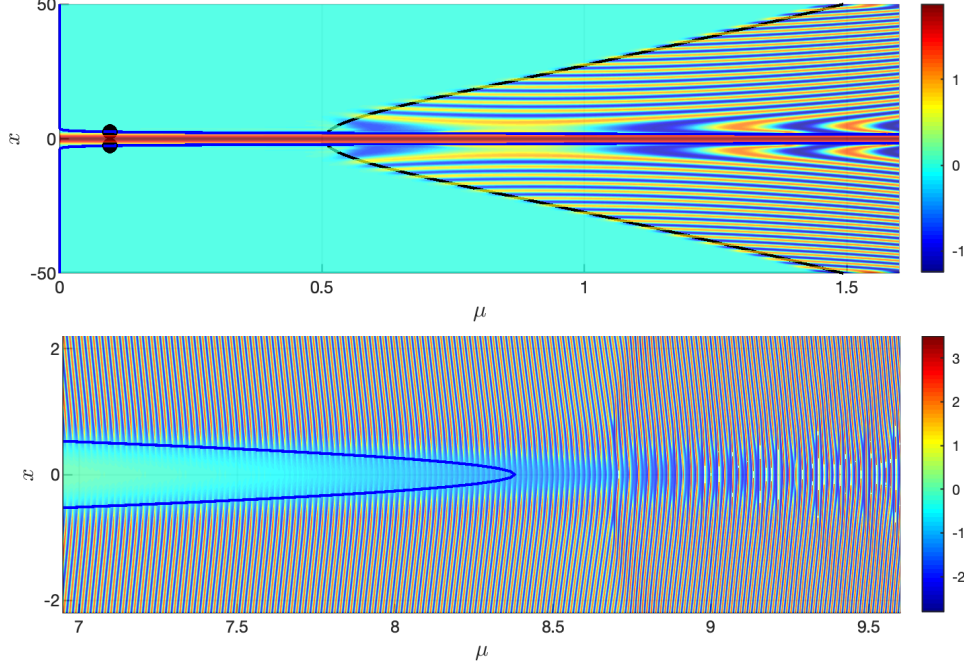
Figure 20: \text{Re}(A(x, \mu)) obtained from (9.1) with Gaussian source term. The QSS has large amplitude in an interval about x = 0 . The space-dependent Hopf curve is given by \mu_{\text{Hopf}}(x) = (8.3788\dots)e^{-\frac{2x^2}{3}} (blue curve). The points x where \mu_{\text{Hopf}}(x) = \sqrt{\varepsilon} are marked by the dots in the upper frame. The curve \mu_{\text{Hopf}}(x) extends to \mu = 8.3788\dots , as is shown in the lower frame. By the time \mu reaches the tip of the Hopf curve, the amplitude of the QSS has decreased (from red to light green and blue). Inside the central interval, the oscillations set in after \mu crosses the blue curve. In contrast, outside this interval, the oscillations set in at \mu_{\text{stbc}}(x) , to leading order, since \mu_{\text{Hopf}}(x) is negligibly small there (upper frame, where the space-time buffer curve (black curve) is also super-imposed). The parameters are \tilde{a} = 1.0 , \sigma = \frac{1}{4} , \varepsilon = 0.01 , \omega_0 = 0.5 , \alpha = 0.6 , d_R = 3 , and d_I = 1 . The initial data at \mu_0 = -1.5 is A_0(x) = -\sqrt{\varepsilon} \frac{I_G(x)}{\mu_0 + i\omega_0} .
