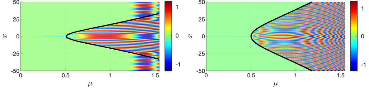
Figure 10: On a finite domain, the parameter \varepsilon changes the width of space-time buffer curve. Here, we fix the values of all of the parameters (except \varepsilon ) to be the same as in Figure 9. Then, in comparison with Figure 9 where \varepsilon = 0.01 , we observe that (a) for \varepsilon = 0.025 the space-time buffer curve is narrower, since at any point x the duration of the DHB \mu_{\text{stbc}}(x) increases as \varepsilon gets larger, by (3.9). Conversely, (b) for \varepsilon = 0.005 , the space-time buffer curve is wider, since at any point x the duration of the DHB \mu_{\text{stbc}}(x) decreases as \varepsilon gets smaller. In fact, for this smaller value of \varepsilon , \mu_{\text{stbc}}(x) < \mu_h(x) for all x on the domain, and the solution has shifted over to being in Case 1 of DHB with this domain.
