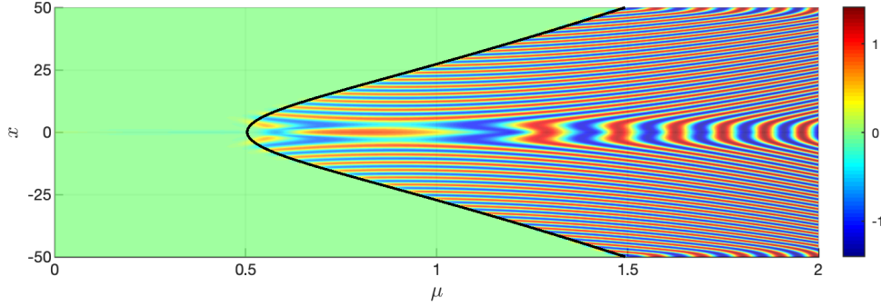
Figure 5: \text{Re}(A(x, \mu)) obtained from (1.1) with source term I_G(x) . In the green region, the solution lies close to the repelling QSS. Superimposed is the black space-time buffer curve obtained by solving (3.8) with g given by (3.11). The oscillations commence just before the space-time buffer curve, where they have small amplitude. Beyond it, the oscillations have large amplitude, since the amplitude of the stable limit cycles is large by this time. The maxima and minima of the oscillations propagate to the center of the interval, toward x = 0 , where they disappear. (The phase velocities and group velocities of the periodic waves are calculated in Section 11.2, where the nature of the defect is studied.) The instantaneous Hopf bifurcation occurs at \mu = 0 to leading order at all x . Here, \varepsilon = 0.01 , \omega_0 = \frac{1}{2} , d_R = 3 , d_I = 1 , \alpha = 0 , and \sigma = \frac{1}{4} . The initial data at \mu_0 = -1.5 is A_0(x) = -\sqrt{\varepsilon} \frac{I_G(x)}{\mu_0 + i\omega_0} . Examples with other initial data are presented below.
