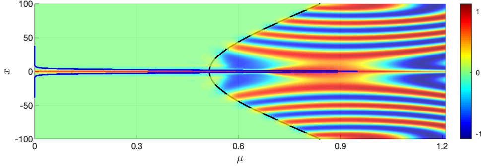
Figure 21: \text{Re}(A(x, \mu)) for the solution of (10.1) on the spatial interval [-100, 100] . The black space-time buffer curve is obtained by solving (10.10) numerically with g given by (10.11), and the blue Hopf bifurcation curve is obtained from formula (10.6) and (10.2). The \mathcal{O}(1) QSS is green in most of the region to the left of the space-time buffer curve, where it has small amplitude; and the QSS is red in the center, where it has maximum amplitude. The parameters are \varepsilon = 0.01, \omega_0 = \frac{1}{2}, \hat{d}_R = 1, \hat{d}_I = 0, \alpha = 0.6 , and \mu_0 = -1 , with I_G(x) = e^{-\frac{x^2}{4\sigma}} , and \sigma = \frac{1}{4} .
