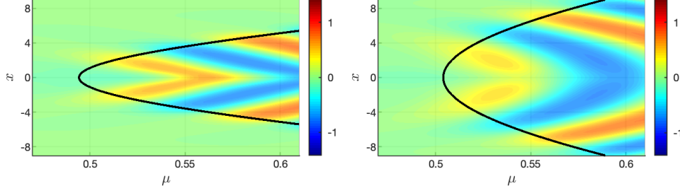
Figure 13: Onset of oscillations near the tip of the space-time buffer curve, of (2.1) in a neighbourhood of x = 0 in the base case \beta = 1/2 and \gamma = 1 of (1.1) with Gaussian source ( \sigma = \frac{1}{4} ). By (7.3), \mu_{\text{Hopf}}(x) = \frac{2\varepsilon(I_G(x))^2}{\omega_0^2} + \mathcal{O}(\varepsilon^2) . The maximum is at x = 0 , and \mu_{\text{Hopf}}(x) decays rapidly for |x| > 0 . Hence, near x = 0 , the delay in the onset of oscillations at each x is slightly longer, creating the “fork in the tongue”. In contrast, away from the center of the domain, the magnitude of \mu_{\text{Hopf}}(x) is negligible, and hence the space-time buffer curve (3.13) determines the DHB and the delayed onset of the oscillations there. Also, this figure illustrates the effect of the logarithmic terms at \mathcal{O}(\varepsilon) in (3.9) and (3.13). Namely, (a) with d_R = 1 and d_I = 0 , the entire buffer curve is shifted leftward from \mu = \omega_0 = \frac{1}{2} by an \mathcal{O}(\varepsilon) amount, as is most visible near the tip, and (b) with d_R = 3 and d_I = 1 , the logarithmic terms shift the buffer curve rightward. The parameters are \varepsilon = 0.01 , \omega_0 = \frac{1}{2} , and \alpha = 0 . The initial data at \mu_0 = -1 is A_0(x) = -\sqrt{\varepsilon} \frac{I_G(x)}{\mu_0 + i\omega_0} .
