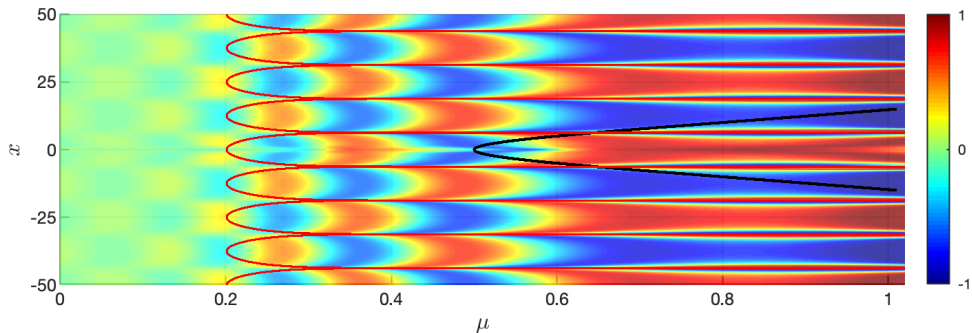
Figure 12: Illustration of DHB in Case 4 with I_G(x) and initial data A_0(x) = \cos(n\pi x/\ell) with n = 4 and \ell = 50 , given at \mu_0 = -0.2 . For all x , the exit time for solutions of the CGL PDE (1.1), is \mu_h(x) (red curve), as determined by A_h . We observe that that \mu_h(x) \sim -\mu_0 = 0.2 , and the \mathcal{O}(\varepsilon) corrections are spatially periodic. The temporal oscillations which set in after \mu_h(x) are stationary in space; there are no propagating pulses. The parameter values are \varepsilon = 0.01, \omega_0 = \frac{1}{2}, d_R = 1, d_I = 0 , and \alpha = 0.6 . The space-time buffer curve (black curve) is super-imposed to illustrate that \mu_{\text{stbc}}(x) plays no role in the onset of the oscillations.
