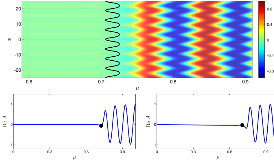
Figure 7: \operatorname{Re}(A) for the solution of (1.1) with the spatially-periodic source term, I_{\text{per}}(x) , p_1 = \frac{1}{3} , and p_2 = \frac{1}{4} . The space-time buffer curve obtained by setting |A_p(x, \mu)| = \sqrt{\varepsilon} is super-imposed (black curve). Time series at x = 5\pi (a local minimum of I_{\text{per}}(x) ) and x = 6\pi (a local maximum) are also shown. The initial data at \mu_0 = -1 is A_0(x) = -\sqrt{\varepsilon} \frac{I_{\text{per}}(x)}{\mu_0 + i\omega_0} . Here, \varepsilon = 0.01 , \omega_0 = 0.75 , \alpha = 0 , d_R = 1 , and d_I = 0 .
