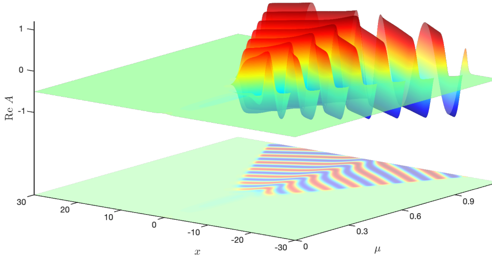
Figure 1: DHB in the PDE (1.1) in the base case of \beta = \frac{1}{2} and \gamma = 1 , with a Gaussian source term I_a(x) = e^{-\frac{x^2}{4}} on the domain [-\ell, \ell] ( \ell = 30 ). The solution is near the attracting QSS while \mu \in [\mu_0, 0) (with \mu_0 = -1 , not shown). Then, for \mu > 0 , i.e. , after the instantaneous Hopf bifurcation, the solution stays near the repelling QSS (green state) at least until \mu = \omega_0 = 0.5 at all points x . The duration of the DHB ( i.e. , the length of time the solution stays near the repelling QSS) is spatially dependent. At x = 0 , A(x, \mu) first leaves a neighbourhood of the repelling QSS at time \mu = \omega_0 , and the large-amplitude oscillations first set in there. Then, as one steps outward from the center, with |x| > 0 , the duration of the DHB grows beyond \mu = \omega_0 . The hard onset of the large-amplitude oscillations is governed to leading order by the space-time buffer curve studied in this article. Here, \varepsilon = 0.01 , \omega_0 = \frac{1}{2} , d_R = 1 , d_I = 0 , and \alpha = 0 .
