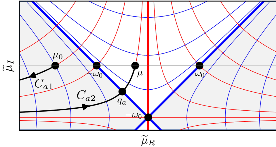
Figure 2: The contour C_a = C_{a1} \cup C_{a2} in the complex \tilde{\mu} plane. Here, and in other figures below, the Stokes lines are the blue curves, and the anti-Stokes lines are the red curves. The Stokes lines through the saddle (thick blue lines) separate the hills (unshaded) and valleys (grey shaded) of the phase function.
