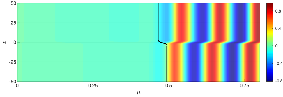
Figure 6: \operatorname{Re}(A(x, \mu)) obtained from (1.1) with the error function source term I_{\text{erf}}(x) , I_{\text{ave}} = 0.5 , and I_e = 0.125 . The black space-time buffer curve is super-imposed, showing that it gives, to leading order, the time of onset of the oscillations at all points x in the domain. Here, the initial data at \mu_0 = -1 is A_0(x) = -\sqrt{\varepsilon} \frac{I_{\text{erf}}(x)}{\mu_0 + i\omega_0} , and the parameter values are \varepsilon = 0.01 , \omega_0 = 0.5 , \alpha = 0 , d_R = 1 , and d_I = 0 .
