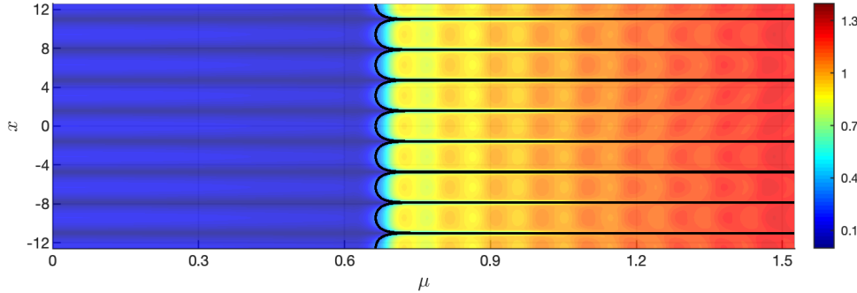
Figure 17: |A(x, \mu)| for the solution of (1.1) with the sign-changing source term, I_{\text{sc}}(x) = \cos(x) . This is an example of Case 2 of DHB. To the left of the exact space-time buffer curve (black curve), the solution is near the small-amplitude, repelling, spatially-periodic QSS. About each point x = k\pi , there is a wide interval on which \mu_{\text{stbc}}(x) < \mu_h(x) , and the hard onset of the large-amplitude oscillations is determined to leading order by the space-time buffer curve. On the narrow, complementary intervals (about x = \frac{(2n+1)\pi}{2} ), \mu_h(x) < \mu_{\text{stbc}}(x) so that the oscillations set in at \mu_h(x) \sim -\mu_0 , as determined to leading order by A_h , and there are \mathcal{O}(\varepsilon) amplitude wiggles about this leading order result, due to the periodicity of the initial data. Here, \varepsilon = 0.01 , \omega_0 = \frac{2}{3} , d_R = 1 , d_I = 0 , and \alpha = 0 . The initial data at \mu_0 = -1 is A_0(x) = -\sqrt{\varepsilon} \frac{I_{\text{sc}}(x)}{\mu_0 + i\omega_0} .
