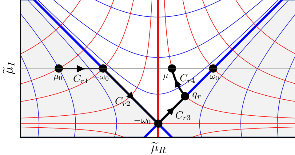
Figure 3: The contour C_r = C_{r1} \cup C_{r2} \cup C_{r3} \cup C_{r4} in the complex \tilde{\mu} plane.
