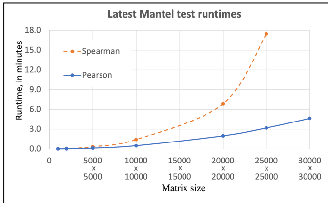
Fig. 3. Measured runtimes for computing a Mantel test using the latest implementation on an Intel Core i7-8565U mobile CPU.
