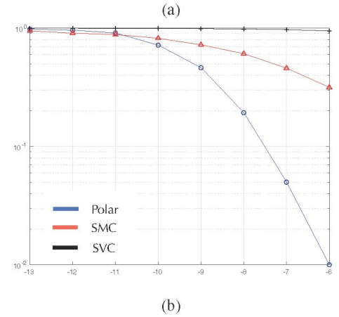
Fig. 4: Performance comparison of SMC with Polar and SVC. Shorter block-lengths are used for SMC compared to Polar and SVC in both (a), (b), but at the same rate. In plot (a) we set \rho_{\text{svc}} = 1024 , \rho_{\text{polar}} = 1024 and \rho_{\text{smc}} = 800 . In (b) we set \rho_{\text{svc}} = 128 , \rho_{\text{polar}} = 256 and \rho_{\text{smc}} = 104 .
