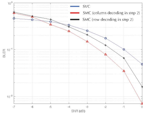
(a) SMC with row-recovery performed first and column-recovery performed first vs SVC
