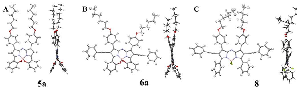
Figure 4. Ellipsoid plots of compounds 5a , 6a , and 8 (front and side views).
