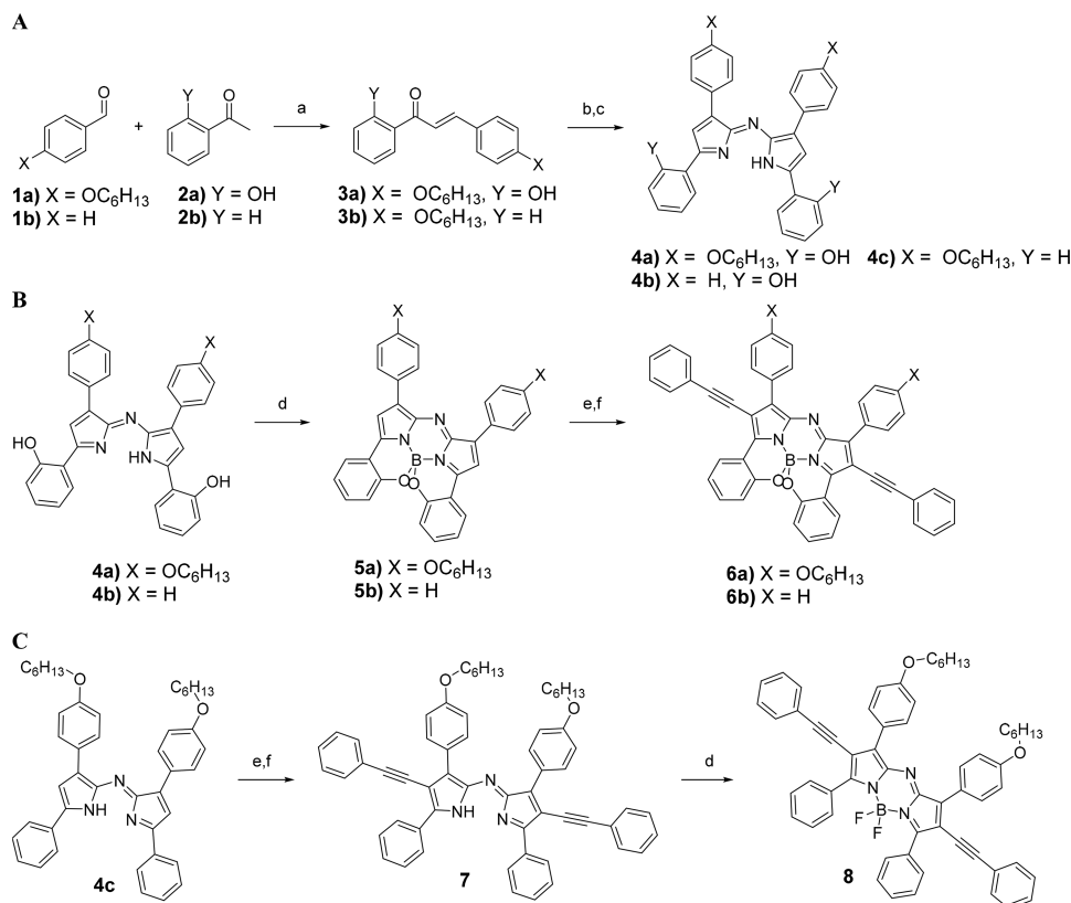
Scheme 1. Synthesis of (A) ADP Compounds, (B) BO-Coordinated Complexes, and (C) the BF 2 Complex a
