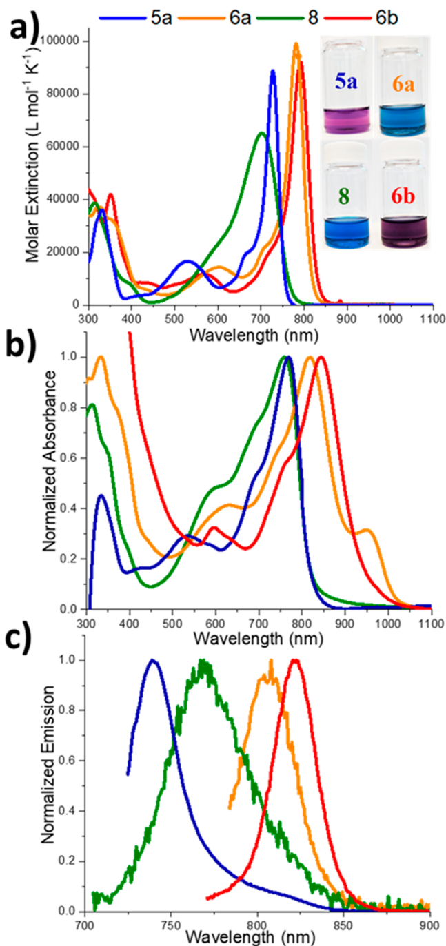
Figure 6. Optical properties of the compounds: (a) UV-vis spectra in \text{CHCl}_3 with solutions in the inset; (b) normalized UV-vis spectra of thin films spin-coated from \text{CHCl}_3 ; (c) normalized fluorescence spectra in \text{CHCl}_3 .
