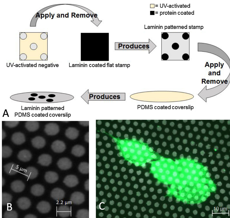
Fig. 1. Hexagonal protein array pattern generation. A) Schematic of patterning protocol. A surface patterned with features that are the inverse of the desired pattern is treated with UV ozone and applied to a laminin-coated PDMS stamp. This results in a PDMS stamp with the desired pattern. This stamp is then applied to a UV ozone-activated PDMS-coated coverslip. B) A representative image of the laminin-patterned surface. C) A representative image of cells (green) attached to the laminin-patterned surface.
