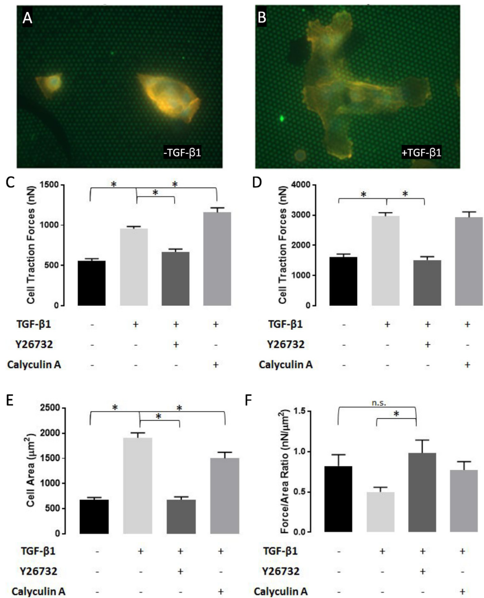
Fig. 4. Comparison and Quantification of Traction Forces in MCF10A cells. A) Representative MCF10A cell on hexagonal pattern. B) Representative MCF10A cell treated with 2 ng/mL TGF-β1 on hexagonal pattern. C) Total cell traction force for area peripheral to cell outline. D) Total cell traction force for areas peripheral to and underneath cells. E) Average cell area F) Total cell force normalized to cell area. * Indicates p-value of <0.05, N > 15.
