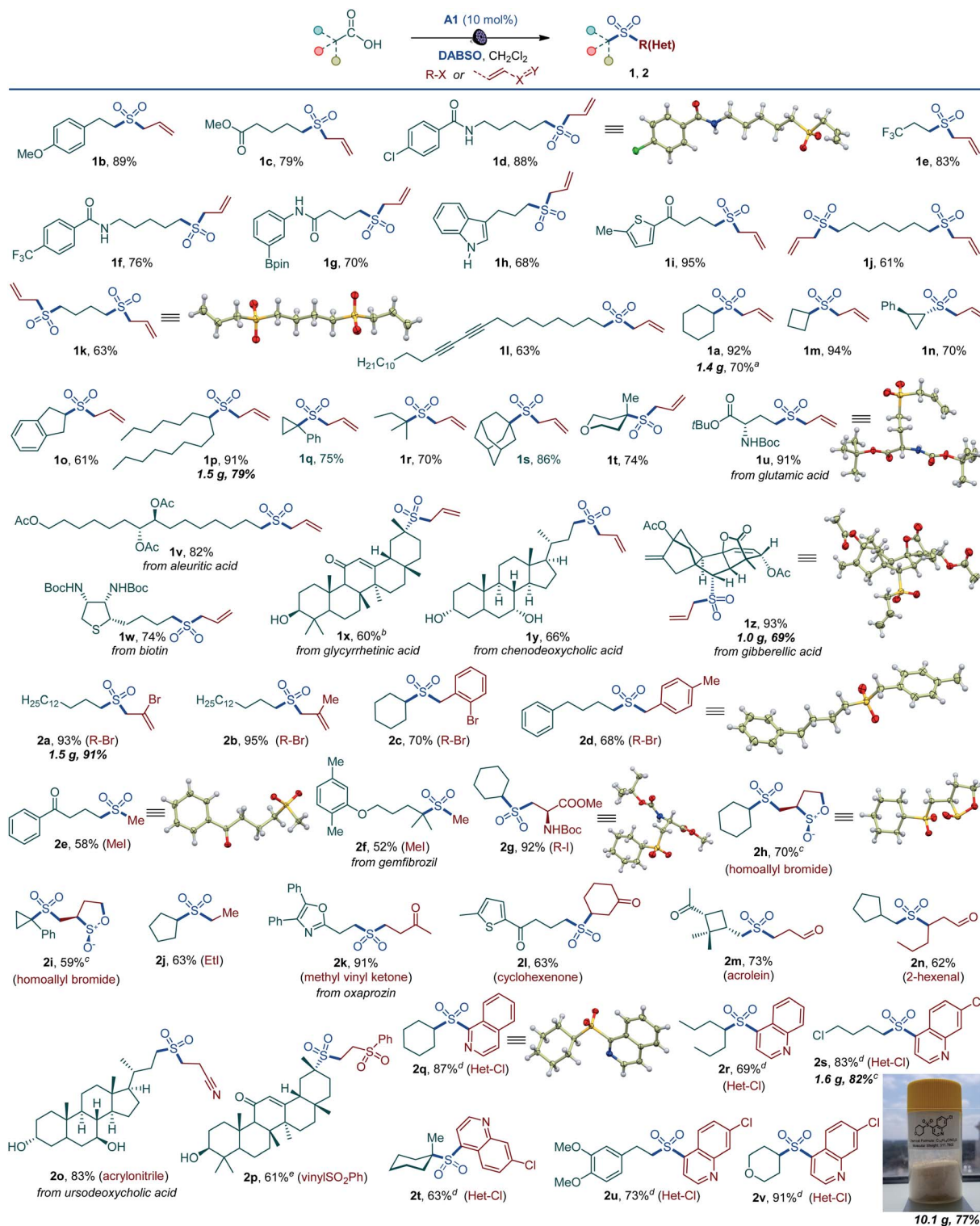
Scheme 1 Scope of the visible light-induced decarboxylative alkylsulfonylation. Reaction conditions: carboxylic acid (0.15–0.3 mmol), DABSO (0.33–0.45 mmol), A1 (10 mol%), alkyl halide (0.75 mmol), \text{CH}_2\text{Cl}_2 (3–6 mL), LED light (400 nm), 12 h. a With \text{Na}_2\text{S}_2\text{O}_5 . b 12 : 1 dr. c cis/trans ratio: 9 : 1. d Halogenated nitrogen heterocycle (0.3 mmol), carboxylic acid (0.75 mmol), DABSO (0.33 mmol), A1 (10 mol%), \text{CH}_2\text{Cl}_2 (6 mL), LED light (400 nm), 12 h. e 19 : 1 dr.
