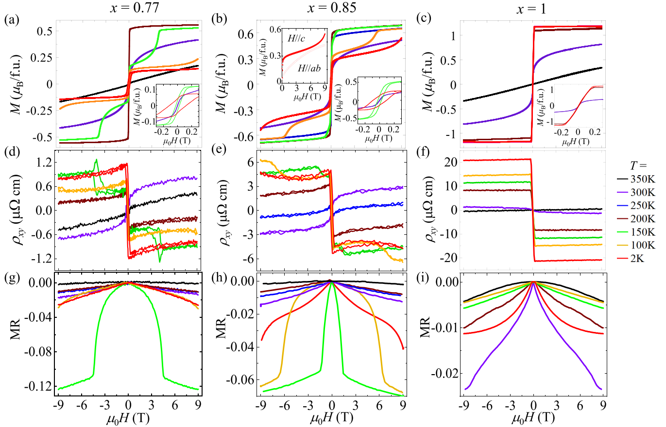
FIG. 3. Magnetic field dependence of (a)–(c) isothermal magnetization M , (d)–(f) Hall resistivity \rho_{xy} , and (g)–(i) normalized magnetoresistivity, MR = [\rho_{xx}(H) - \rho_{xx}(H = 0)]/\rho_{xx}(H = 0) for x = 0.77 , x = 0.85 , and x = 1 samples, measured with \mathbf{H} \parallel c . Metamagnetic transitions below the HT-FI transition temperatures are manifested by the jump at higher fields at 150 K in the x = 0.77 and 100 K in the x = 0.85 sample. For each of those three compositions, identical samples were used for Hall effect and magnetoresistivity measurements. Lower insets in (a)–(c): Zoom-in of the low field magnetization. Upper inset in (b): Out-of-plane ( \mathbf{H} \parallel c ) and in-plane ( \mathbf{H} \parallel ab ) magnetization for the x = 0.85 sample at T = 2 K. The same color code is used for all panels.
