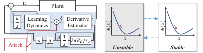
Fig. 1: ES controller under persistent gradient deception. The system is modeled as a switched system with unstable modes.
