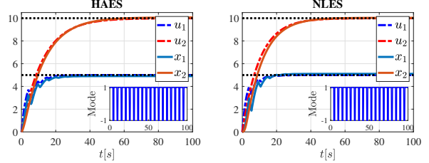
Fig. 3: HAES and NLES under persistent gradient jamming.
