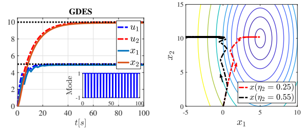
Fig. 2: GDES under persistent gradient jamming.
