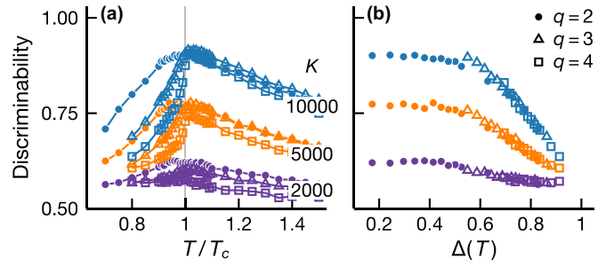
FIG. 7. Interaction discriminability for Ising and Potts models. Discriminability maximum results from the competition between thermal noise and macroscopic ordering but is not a signature of criticality associated with second-order phase transitions. We show DCA discriminability at different sample sizes K (see legend) as a function of temperature (a) and mean-field order parameter \Delta (b). In all cases, discriminability peaks at an intermediate temperature and displays similar temperature dependence above T_c . By plotting discriminability as a function of \Delta for T < T_c , we see that a different temperature dependence for Ising and Potts models at T < T_c originates from the fact that macroscopic order forms more rapidly in Potts models which admit first-order phase transitions. This highlights the detrimental effect of macroscopic order on inference quality. Shown results are based on the same Erdős-Rényi interaction graph with 400 vertices and mean degree 40.
