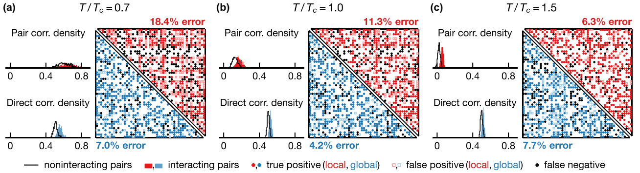
FIG. 2. Local statistical modeling outperforms mean-field DCA in the disordered phase. We show density histograms of empirical and direct pair correlations— \langle\sigma_i\sigma_j\rangle_{\text{data}} and \langle\sigma_i\sigma_j\rangle_{\text{dir}} [see Eq. (5)]—for interacting (filled) and noninteracting (line) pairs of spins at T/T_c = 0.7, 1.0, 1.5 [(a)–(c), respectively]. The predictions of pairwise interactions are depicted in a contact map for local (upper half) and global (lower half) inference. The discrimination threshold is chosen such that the number of positive predictions is equal to the number of real interactions, and false positives and false negatives are equal (see legend). In general, both empirical and direct pair correlations are higher among interacting spins and are thus informative of interactions. For local inference, the prediction error decreases with temperature and is smaller than that of global inference at T/T_c = 1.5 (c). Global inference error exhibits nonmonotonic temperature dependence and is minimal at an intermediate temperature T/T_c = 1.0 (b). Shown results are based on 5 \times 10^3 samples drawn from Ising models on an Erdős-Rényi graph with 50 vertices and mean degree 20.
