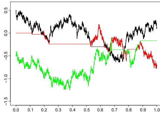
Figure 3. Simulated processes; Black = X_1(\cdot) , Red = X_2(\cdot) , Green = X_3(\cdot) . Here we have taken \delta_1 = -0.5 , \delta_2 = 0 and \delta_3 = 0.5 in (3.1).
