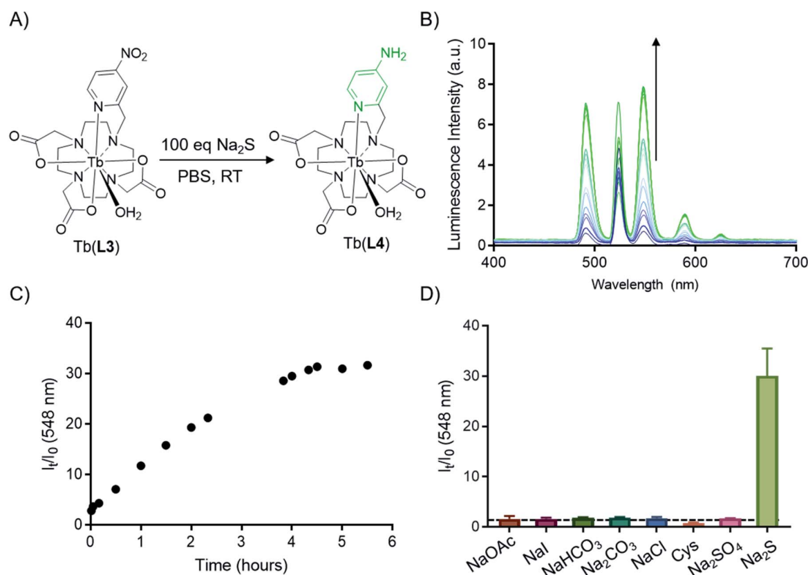
Fig. 4 (A) Reaction scheme of Tb(L3) (10 \mu\text{M} ) reacting with 100 equiv. Na 2 S (1 mM) to form Tb(L4) in situ . (B) Emission spectra over time upon reduction of 10 nmol (10 \mu\text{M} ) Tb(L3) (523 nm peak = scattering). (C) Fold-increase of emission over 5.5 hours. (D) Relative fold-change of emission of 10 nmol (10 \mu\text{M} ) Tb(L3) in response to NaOAc, NaI, NaHCO 3 , NaCl, Na 2 SO 4 , Cys, and Na 2 S (100 equiv.) in PBS (dashed line = 1; error bars represent standard deviation, n = 3 ).
